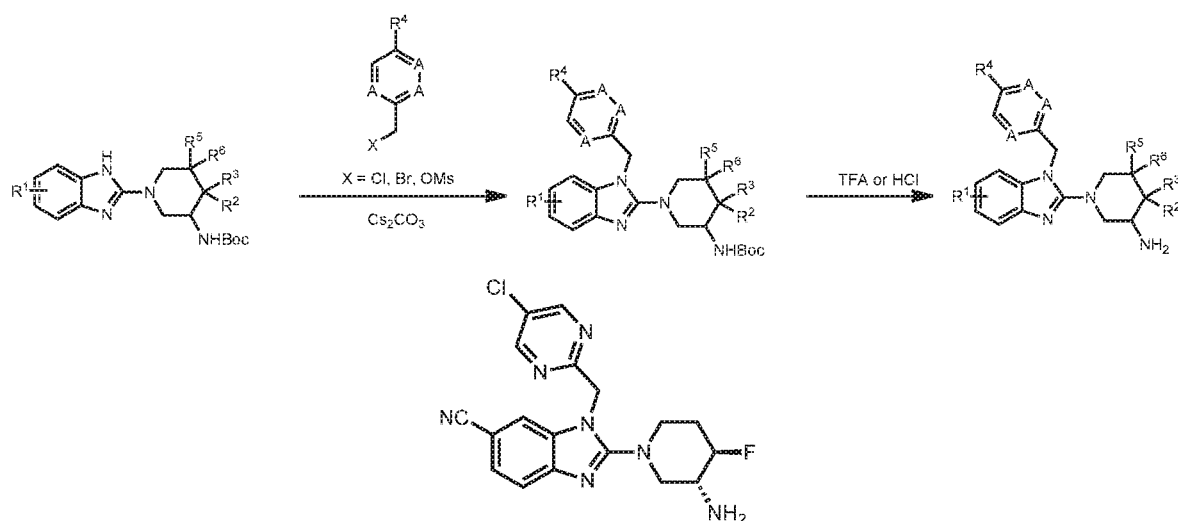
Scheme 10. Advancement of S_NAr intermediates to final products
