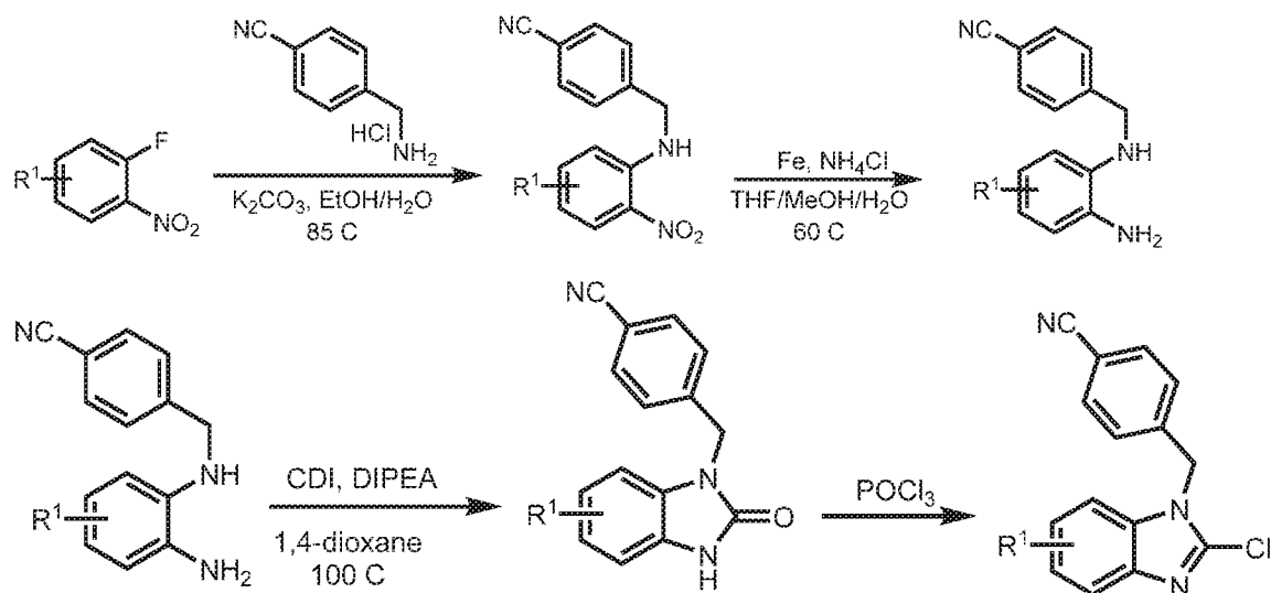
Scheme 11. Accessing chlorobenzimidazoles selectively
