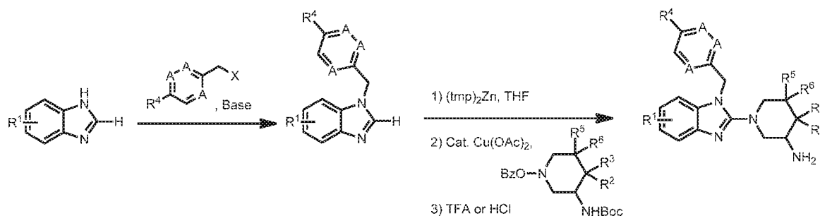
Scheme 6
