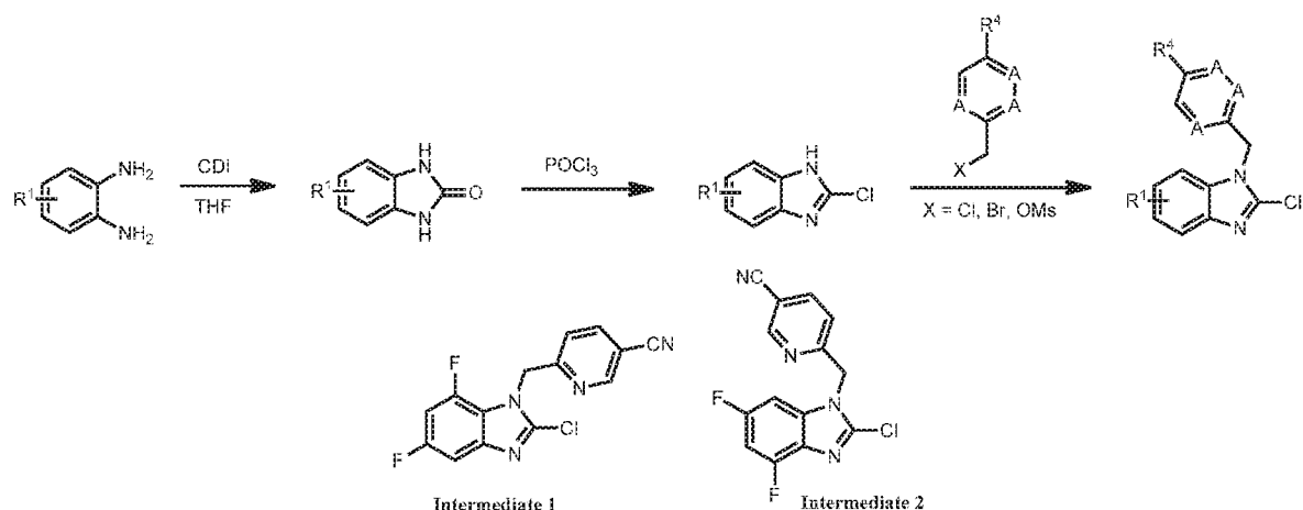
Scheme 7. General Synthesis of Alkylated Intermediates
