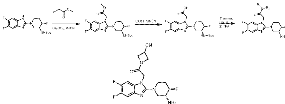
Scheme 14. Compounds made through peptide coupling
