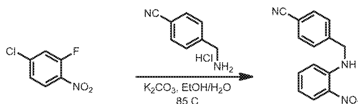
Intermediate 86: 4-((2,6-dichloro-1H-benzo[d]imidazol-1-yl)methyl)benzonitrile
