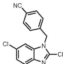
Intermediate 86: 4-((2,6-dichloro-1H-benzo[d]imidazol-1-yl)methyl)benzonitrile
