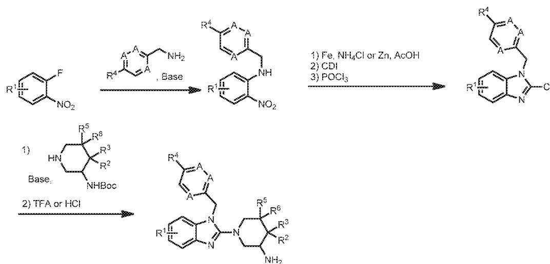
Scheme 7. General Synthesis of Alkylated Intermediates
