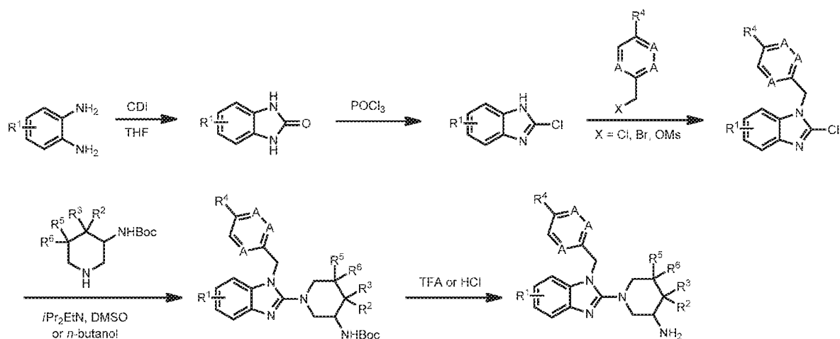
Scheme 1
