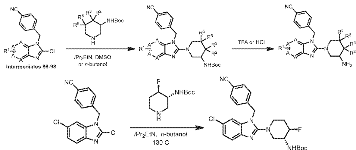
Scheme 12. Advancement of benzylated intermediates to final products
