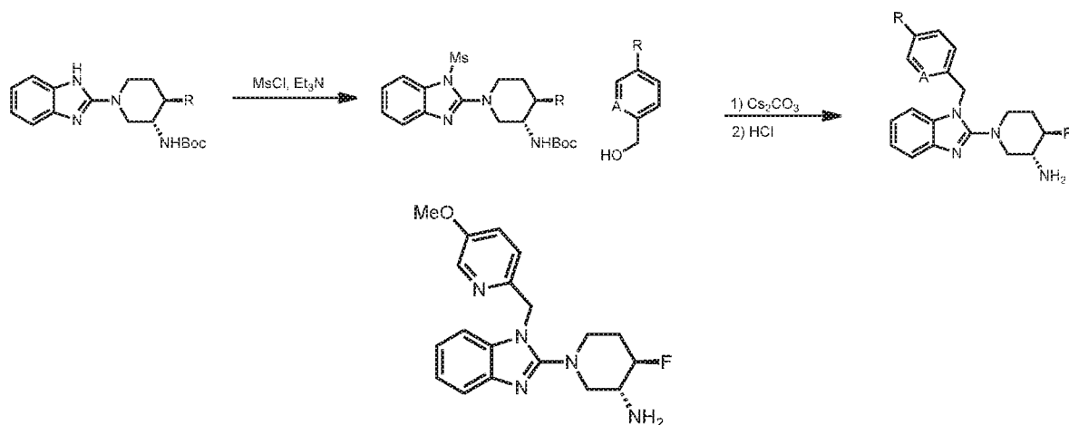
Scheme 13. Mesylate Transfer Chemistry
