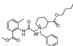
Compound 14A
