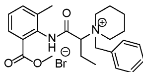
Compound 57
