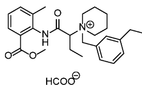
Compound 58A
