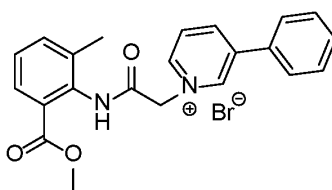
Compound 66A
