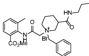
Compound 28A
