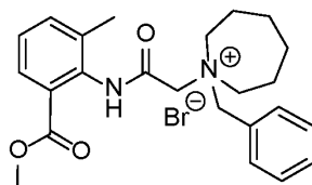
Compound 1A
