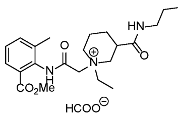
Compound 29A
