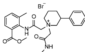
Compound 59A
