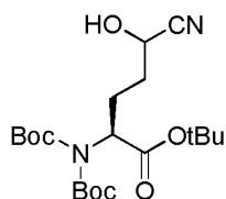
(2S)-tert-butyl 2-(bis(tert-butoxycarbonyl)amino)-5-cyano-5-hydroxypentanoate
