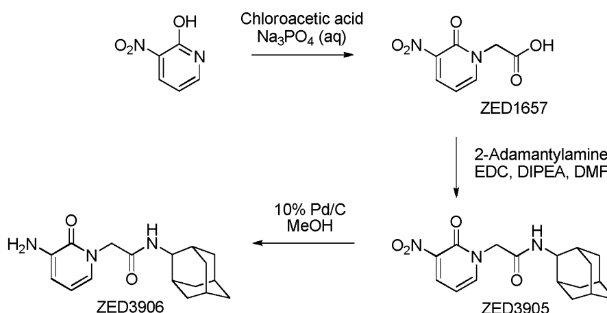
Scheme II-1
