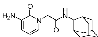
2-(3-amino-2-oxopyridin-1(2H)-yl)-N-(2-adamantyl)acetamide
