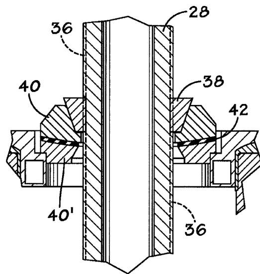
DETAIL B
