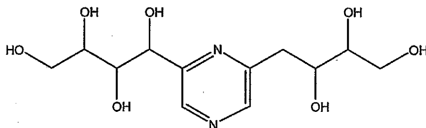
1-[6-(2,3,4-trihydroxybutyl)-pyrazin-2-yl]-butane-1,2,3,4-tetraol (2,6-deoxyfructosazine)
