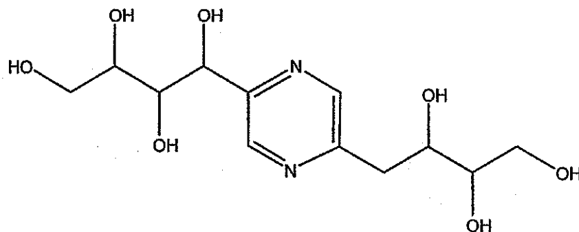
1-[5-(2,3,4-trihydroxybutyl)-pyrazin-2-yl]-butane-1,2,3,4-tetraol (2,5-deoxyfructosazine)
