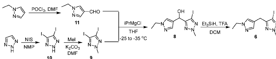
Scheme 1. Synthesis of Compound 6.
