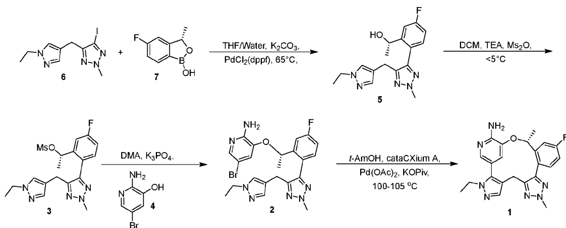
Scheme 3. Synthesis of Compound 1.
