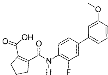
formula (Ia)
