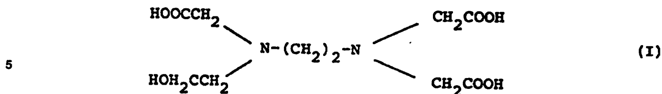
N-Hydroxyethyl-N,N',N'-ethylenediaminetriacetic acid (HEDTA)
