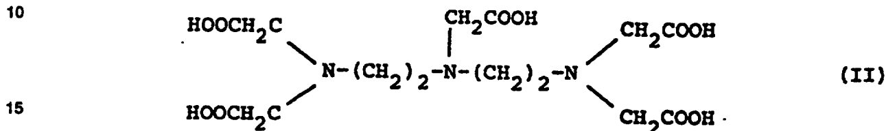
N,N,N',N'',N''-Diethylenetriaminepentaacetic acid (DTPA)
