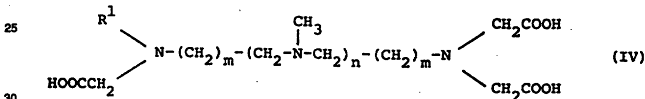
N-Hydroxyethyliminodiacetic acid
