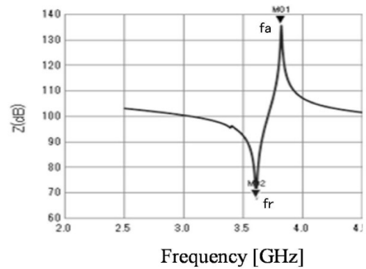
FIG. 6(b) (0^\circ, 132^\circ, 0^\circ) LT/c-sapphire substrate
