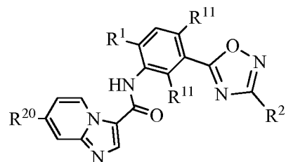
Formula (IIc)
