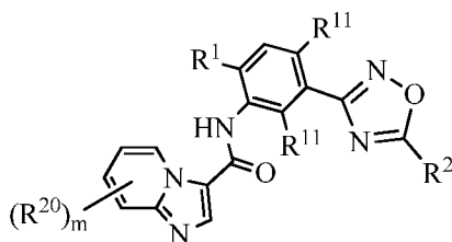
Formula (Ia)
