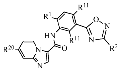
Formula (IId)
