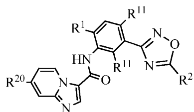
Formula (Ic)
