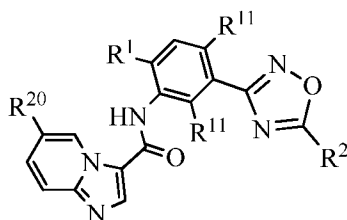
Formula (Ic)
