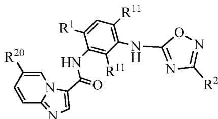
Formula (IIe)
