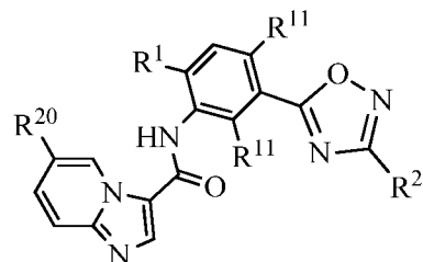
Formula (IIc)
