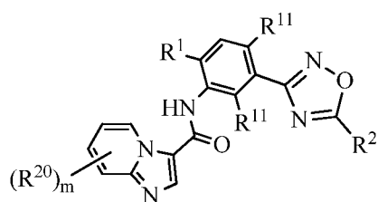
Formula (Ia)
