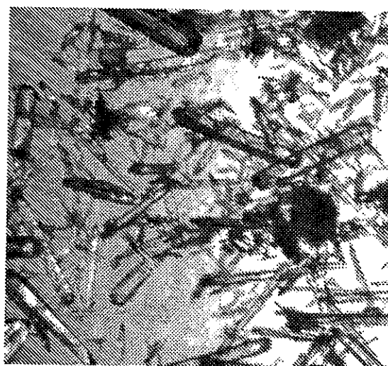
Crystal Form 3
