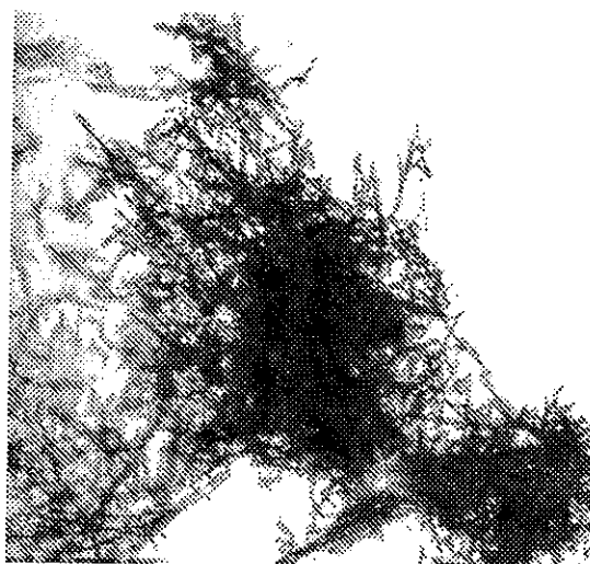
Crystal Form 1
