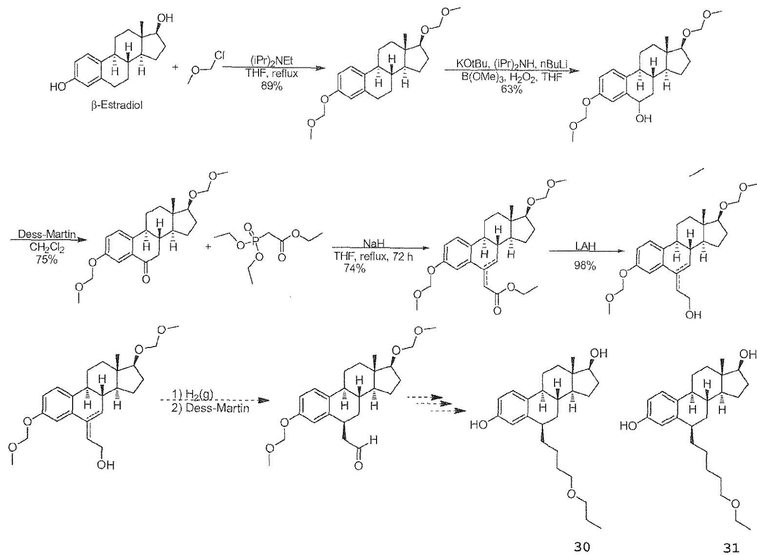
Scheme 4
