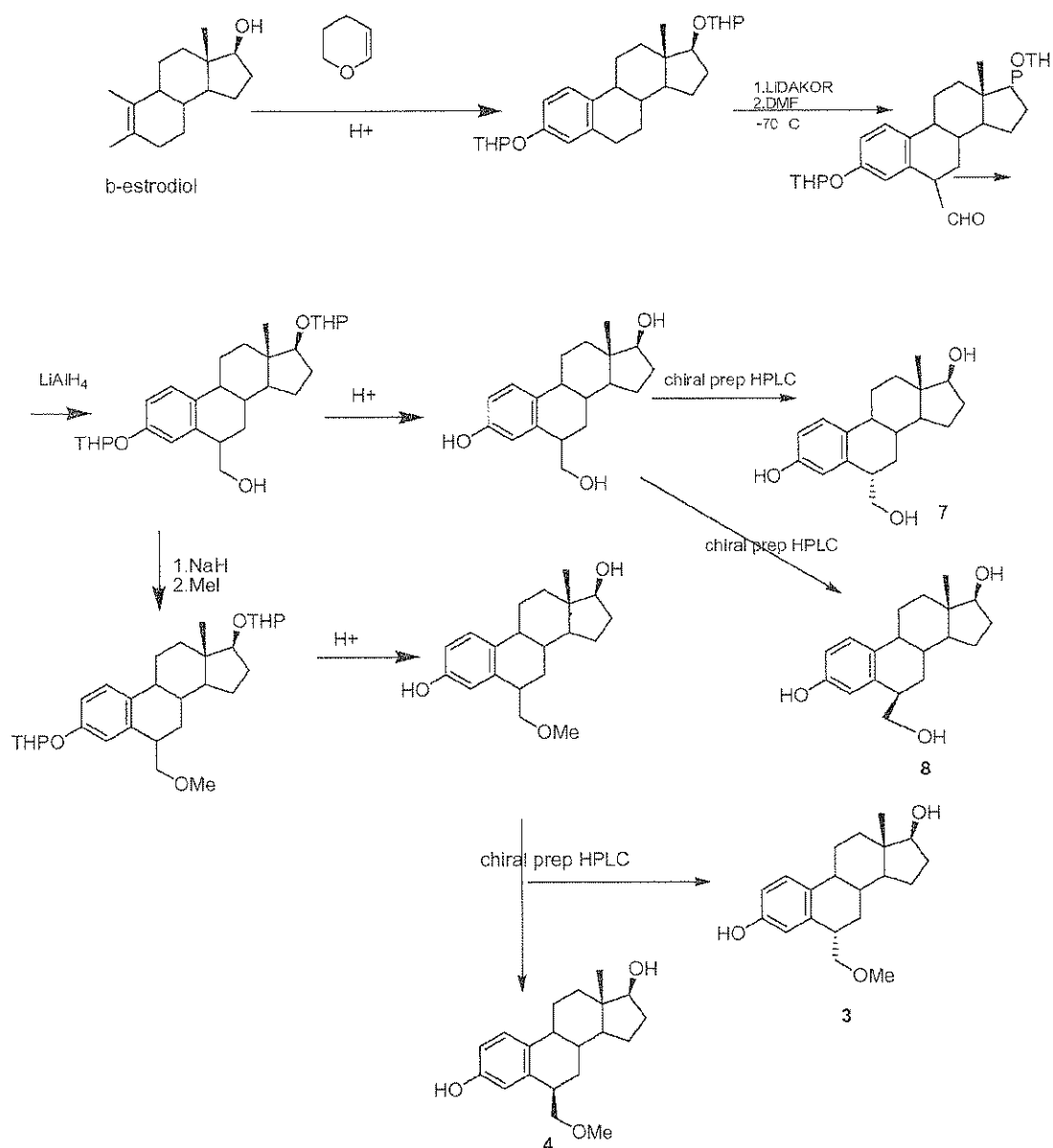
Scheme 2
