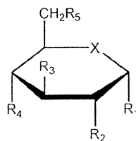
Formula IV
