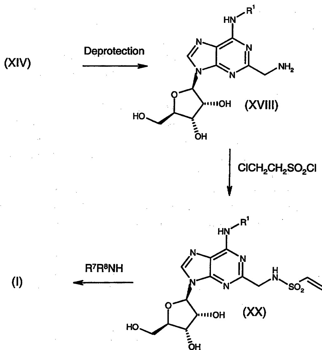
Scheme 4
