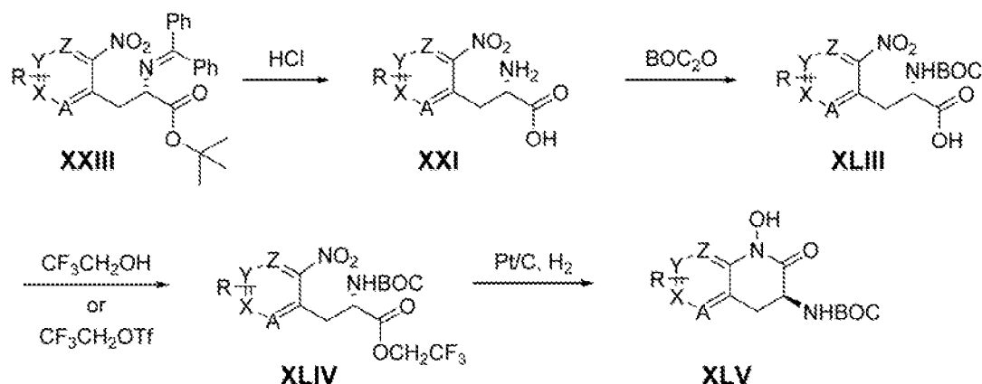
Scheme 11
