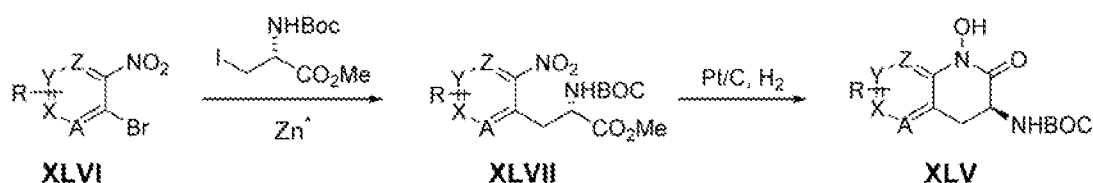
Scheme 12
