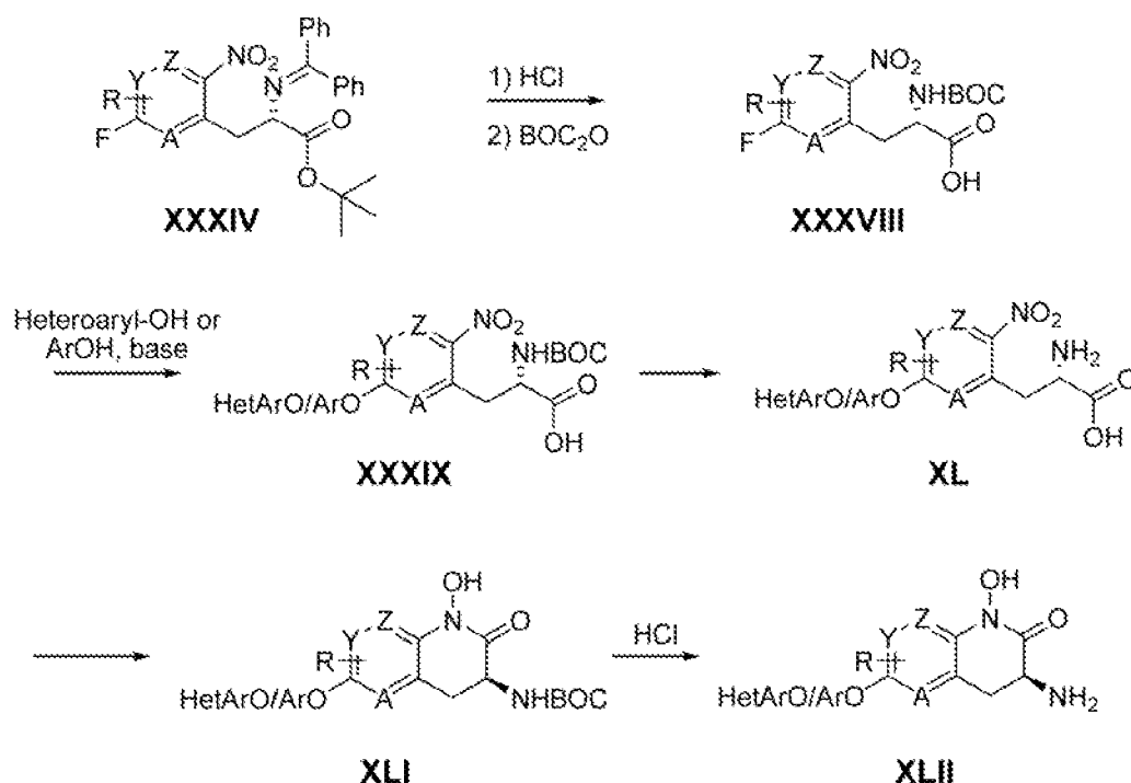
Scheme 10
