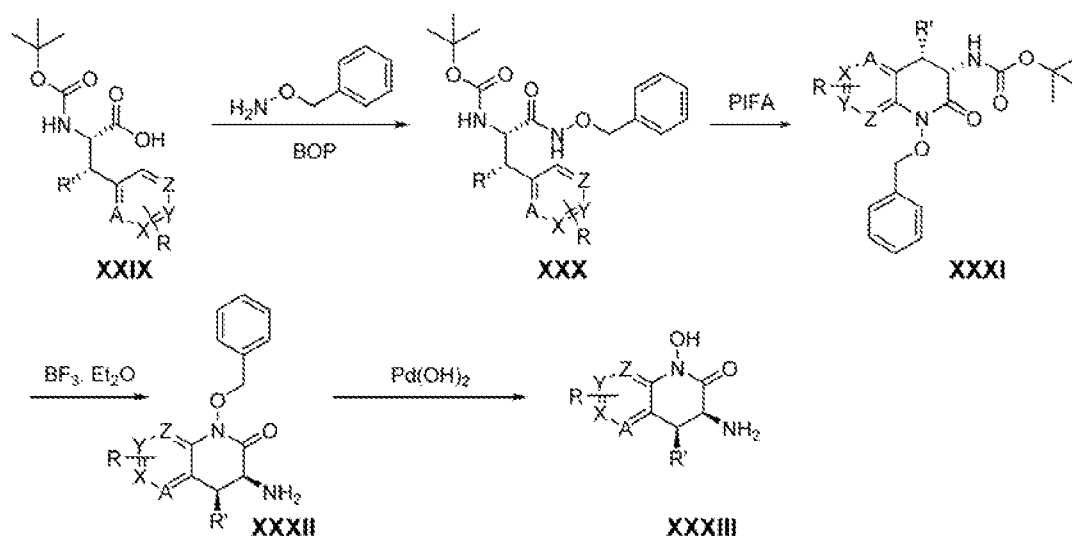
Scheme 8
