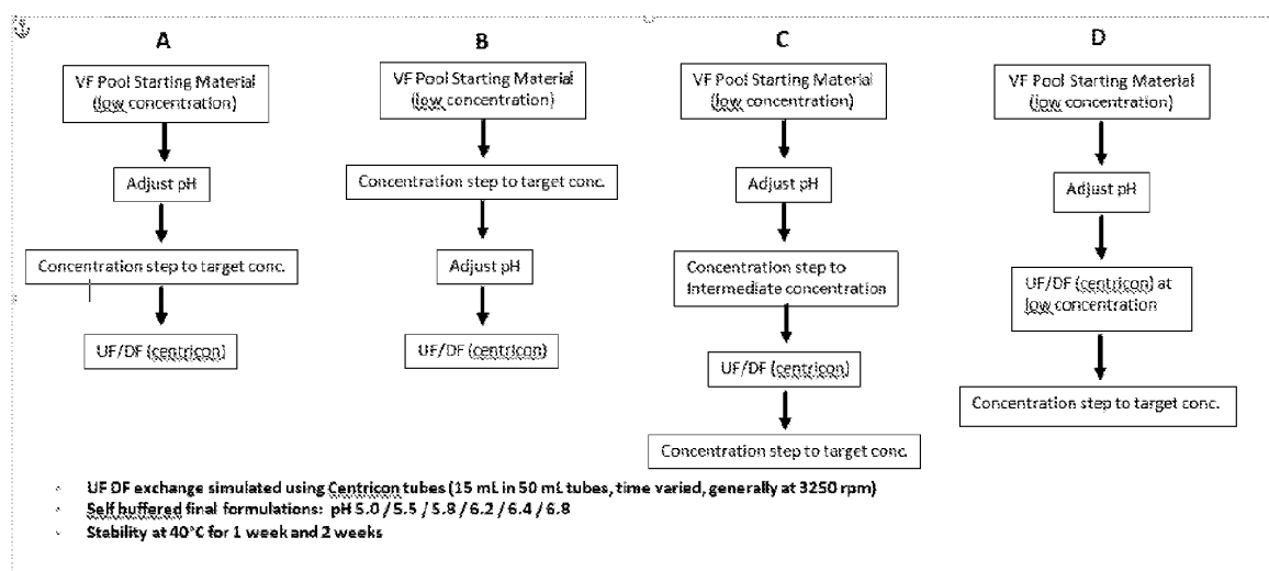
Figure 5. Four manufacturing process options
