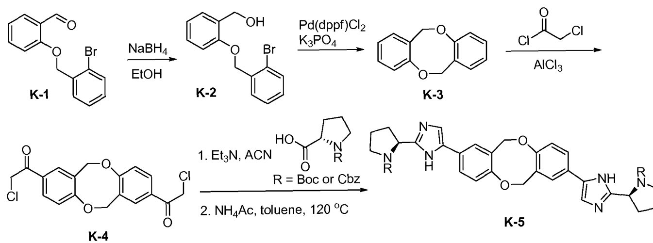
Scheme K
