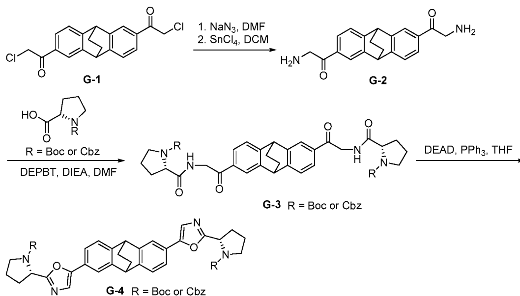
Scheme G
