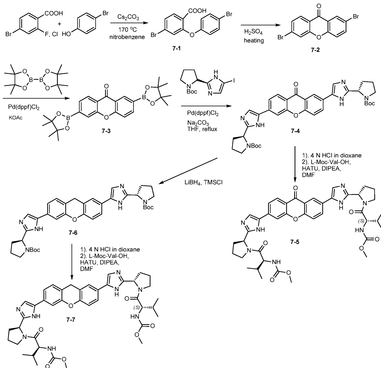
Scheme 7
