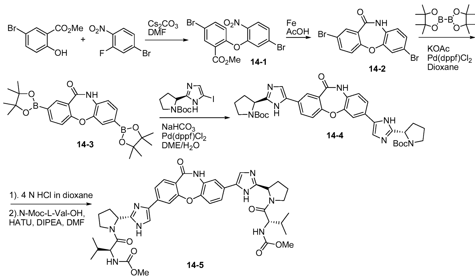
Scheme 14
