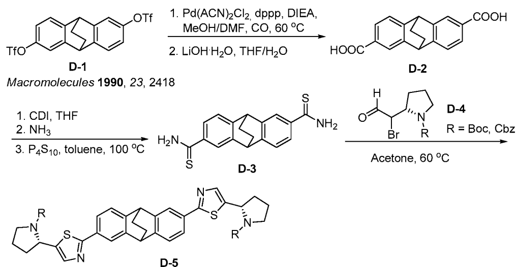
Scheme D
