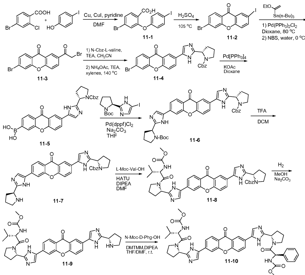
Scheme 11
