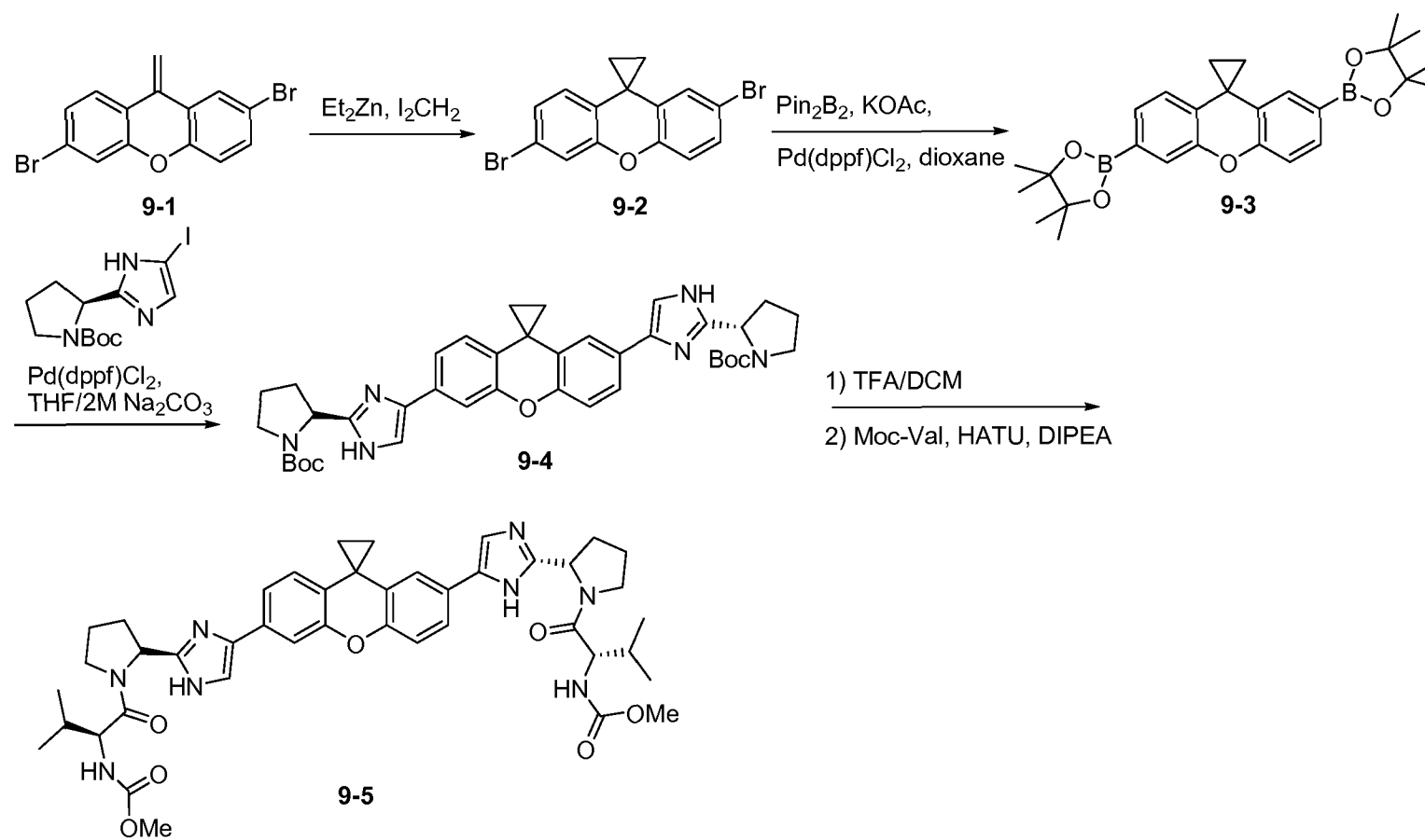
Scheme 9
