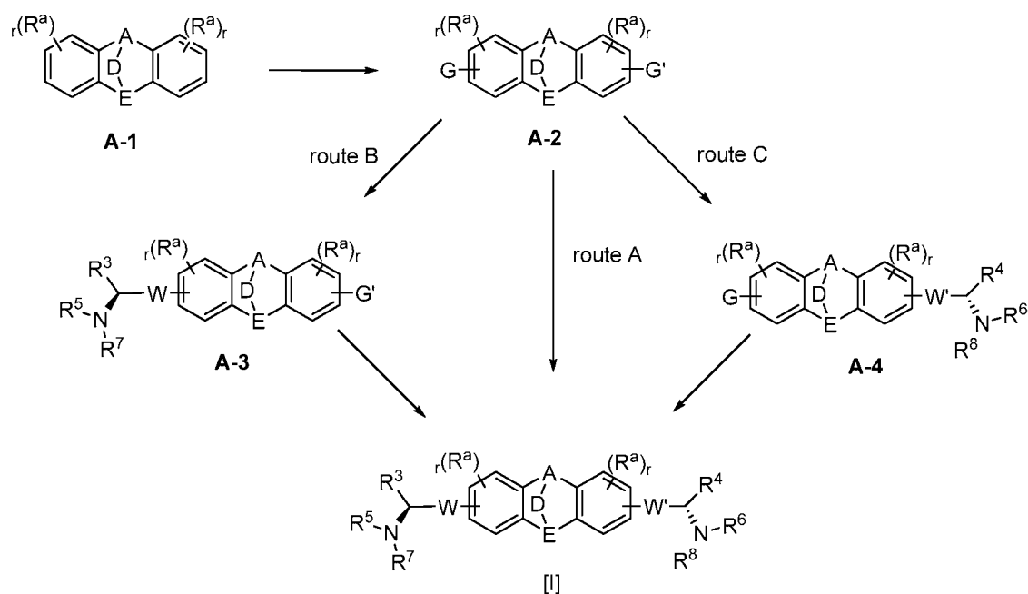
Scheme A
