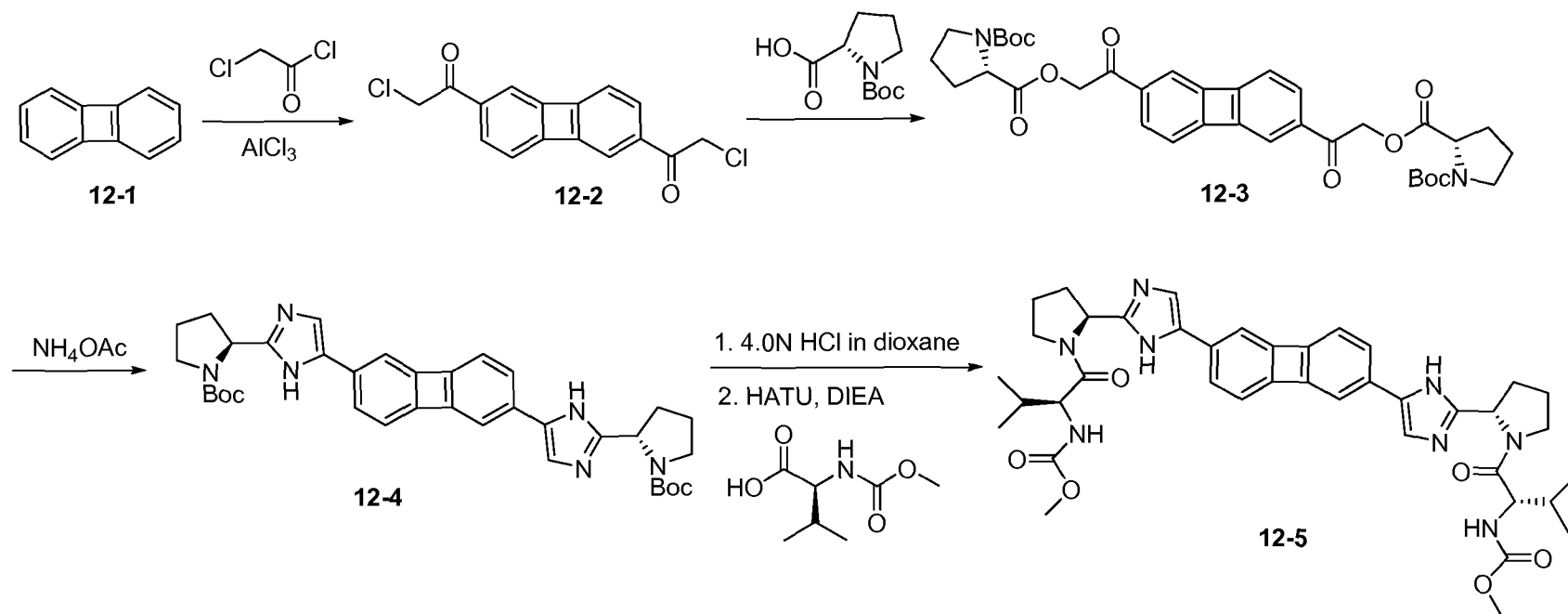
Scheme 12
