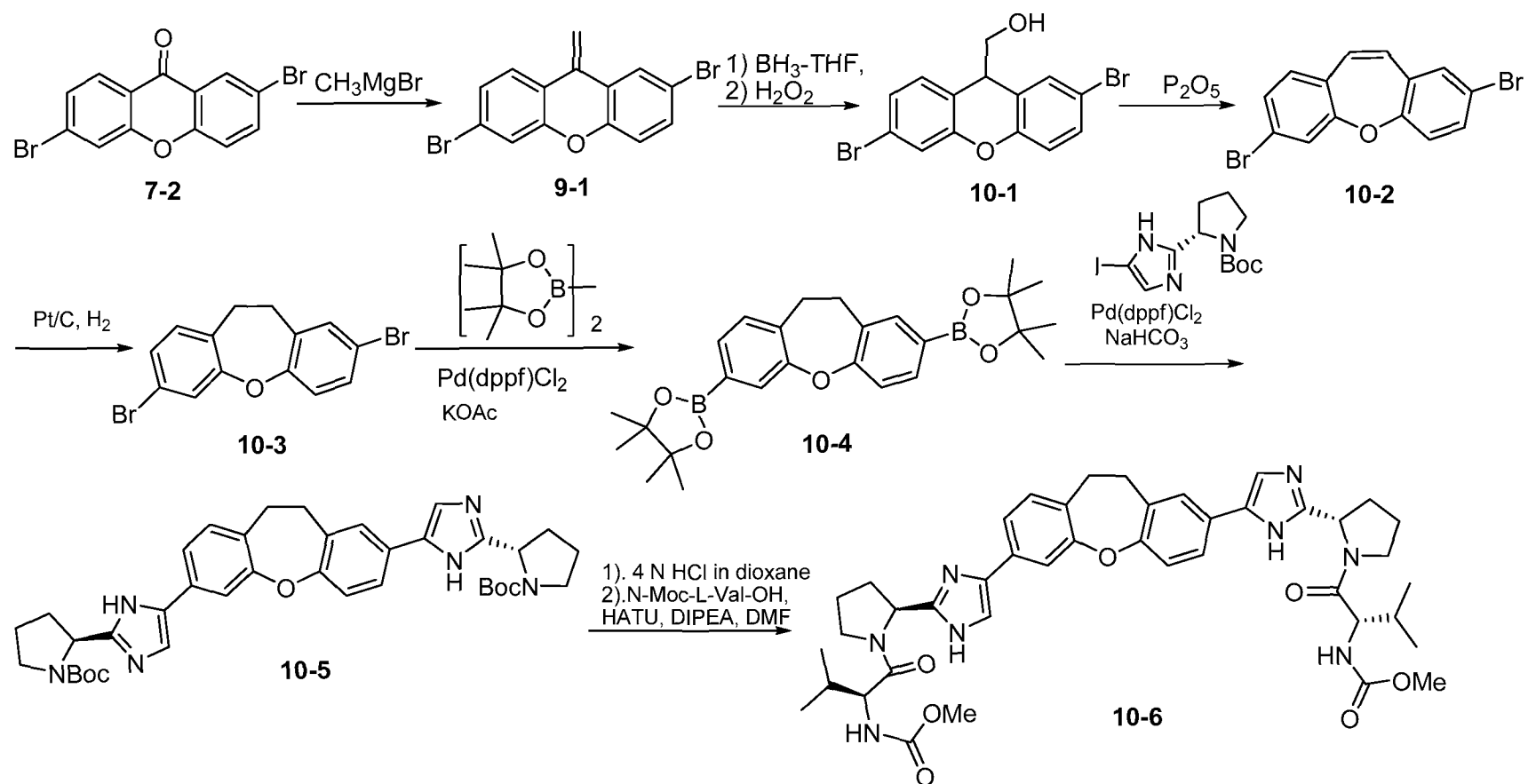
Scheme 10
