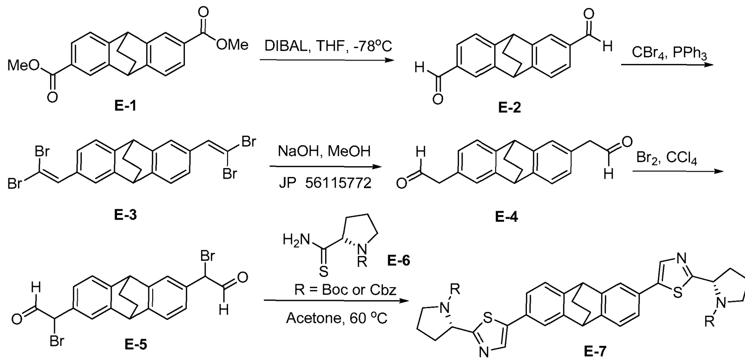
Scheme E
