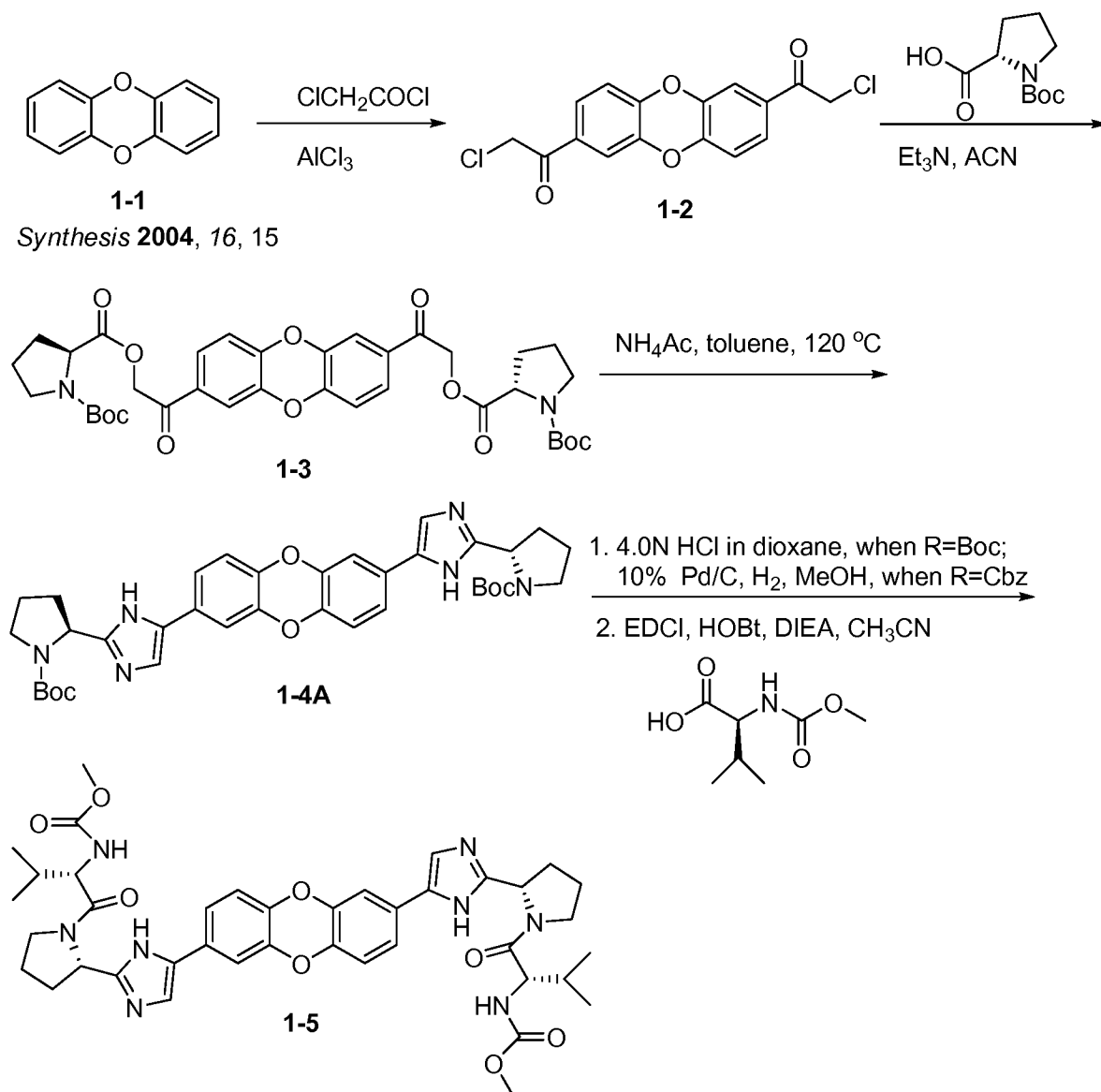
Scheme 1
