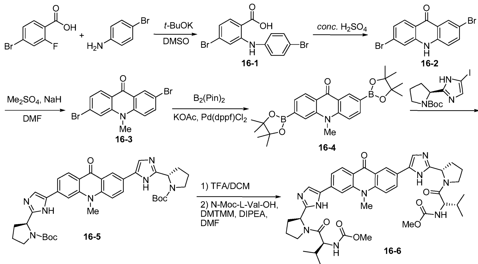
Scheme 16
