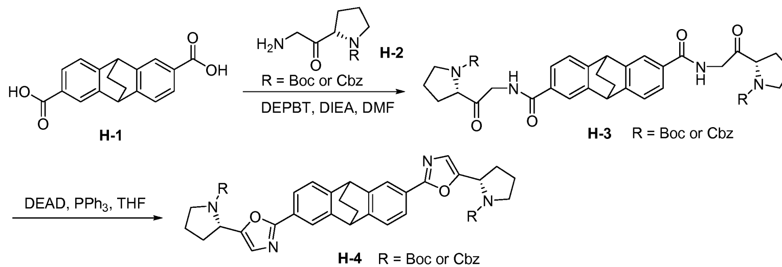
Scheme H
