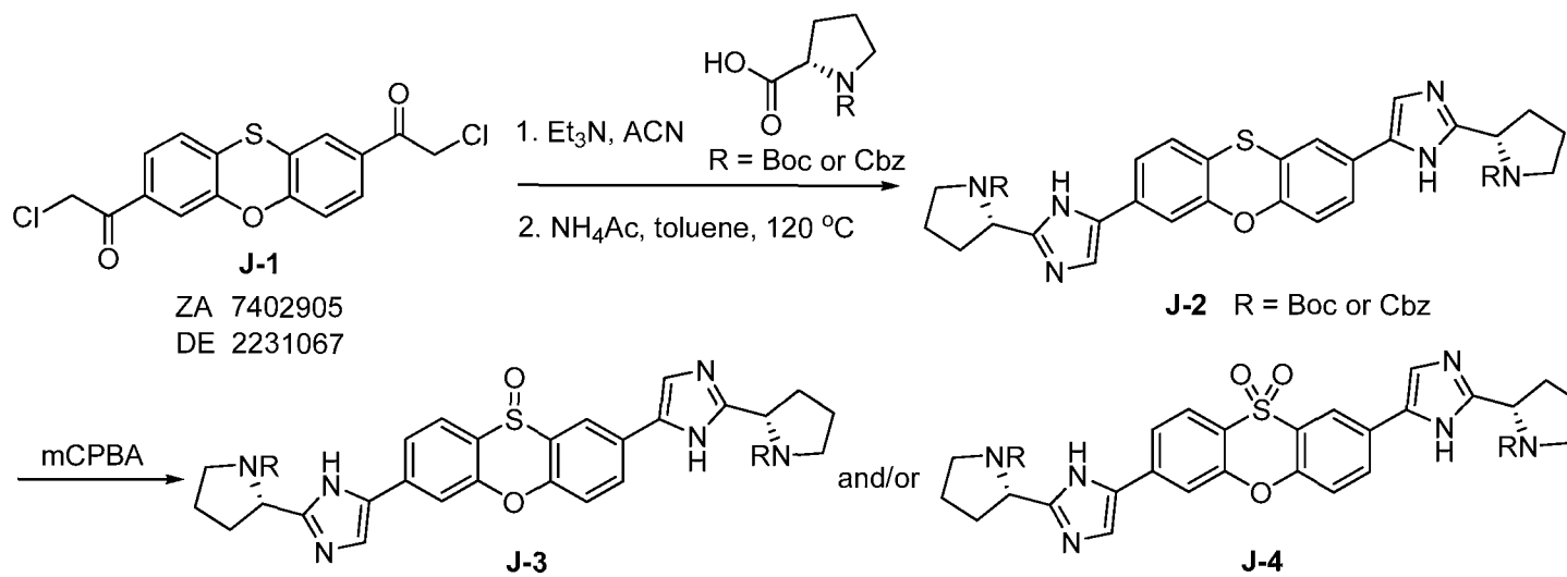
Scheme J
