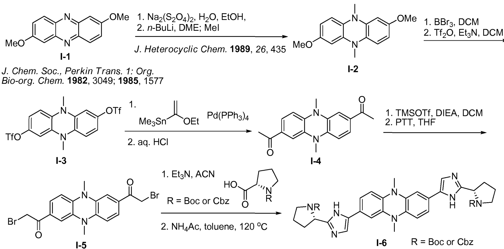
Scheme I
