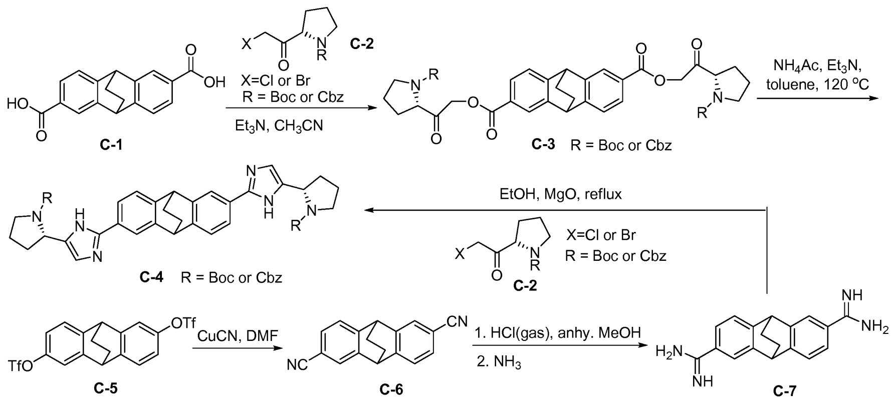
Scheme C
