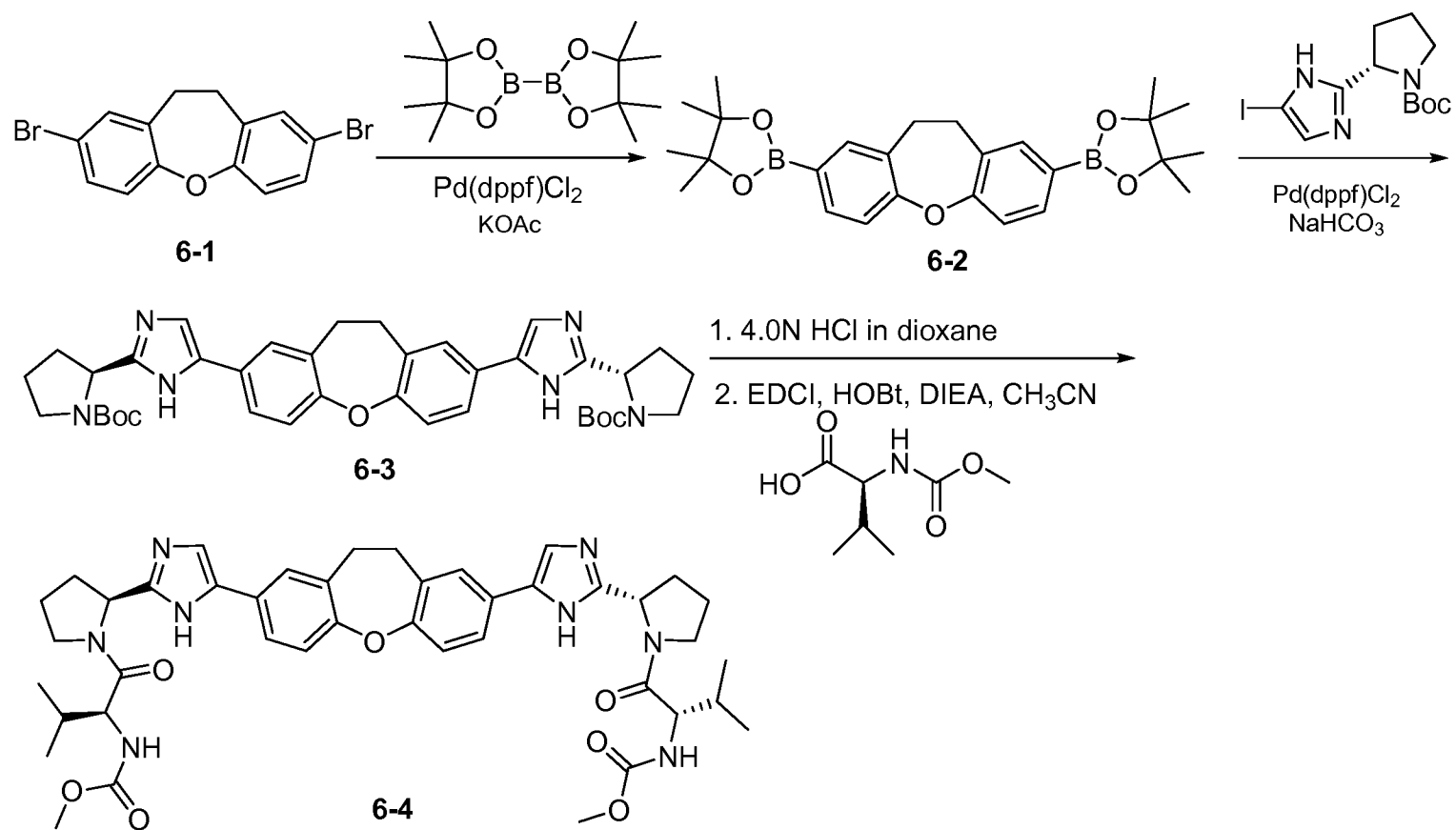
Scheme 6
