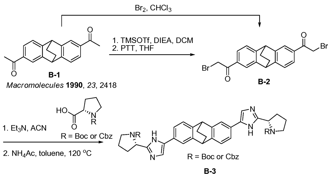
Scheme B
