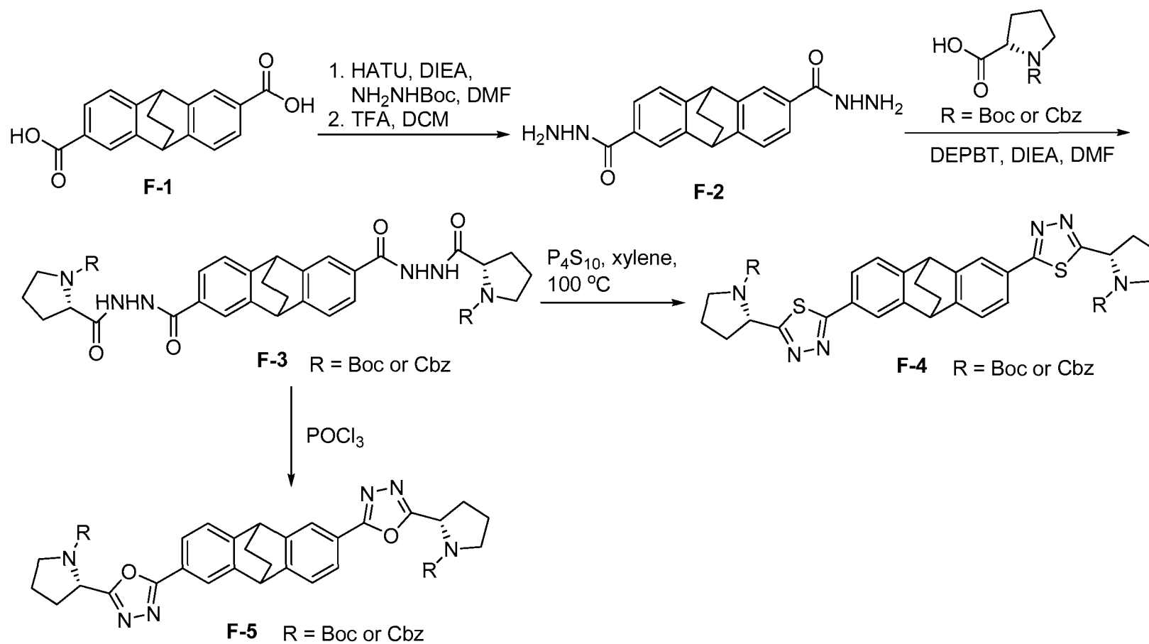
Scheme F
