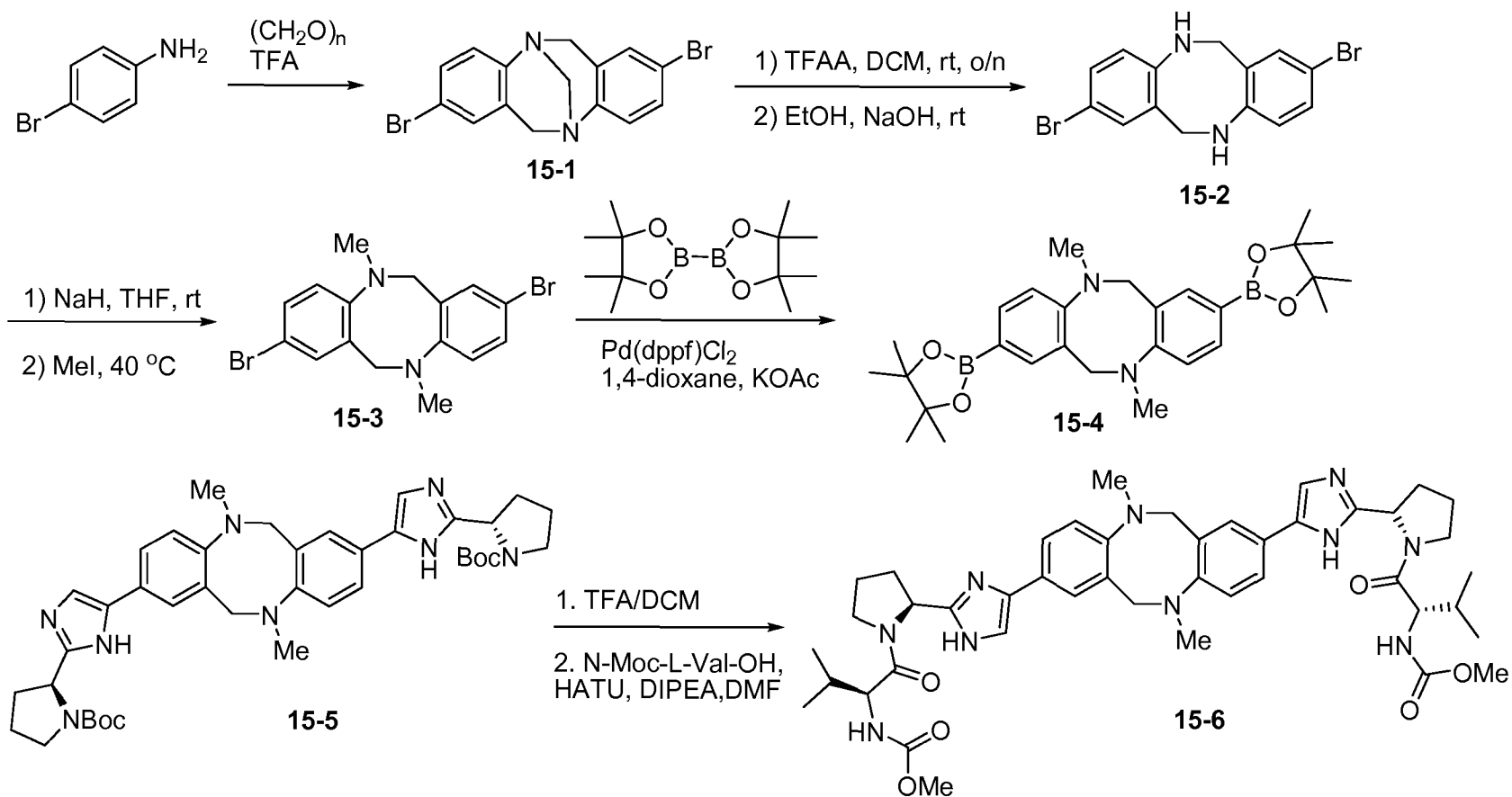
Scheme 15
