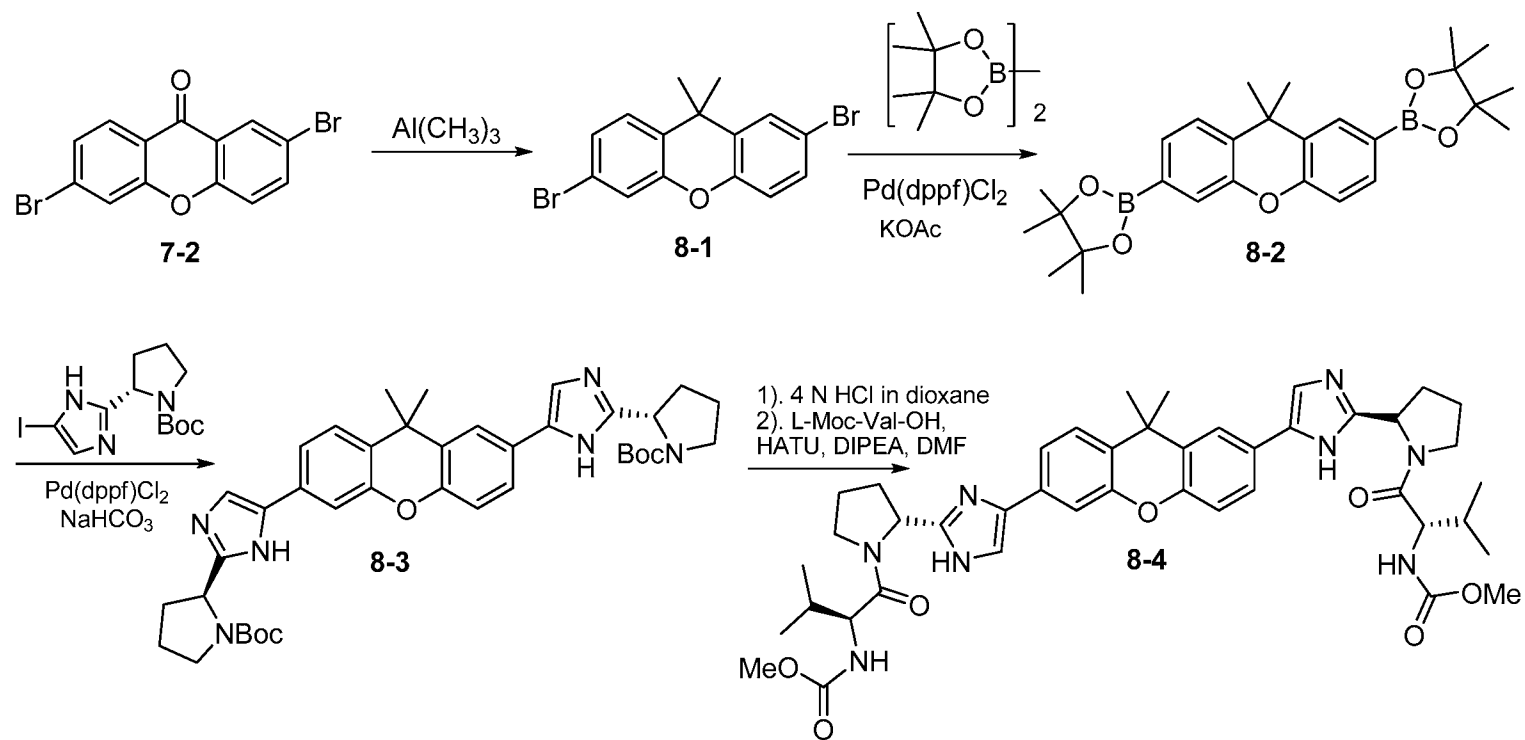
Scheme 8
