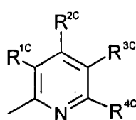
2-pyridyl
