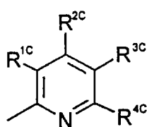
2-pyridyl
