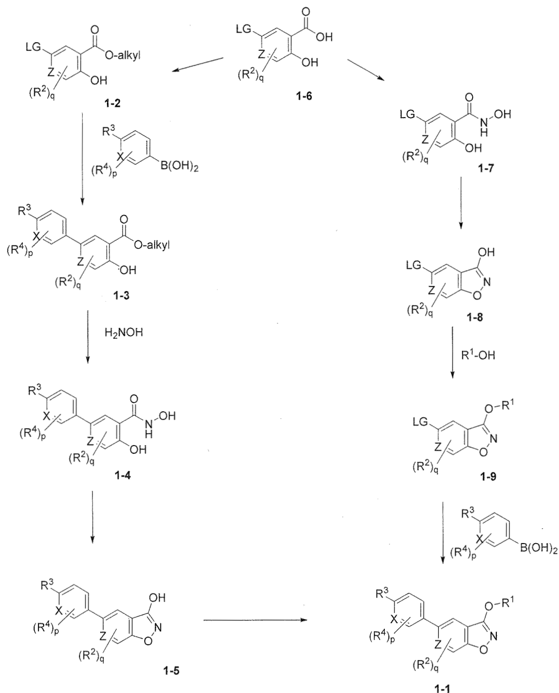
Scheme 1
