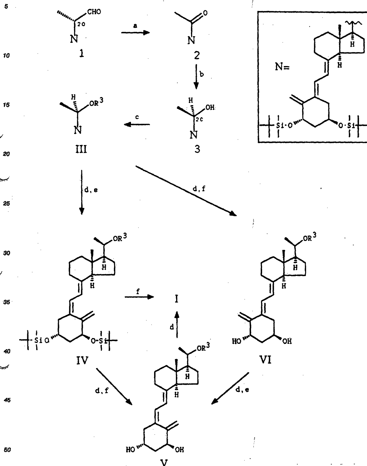
Scheme 1
