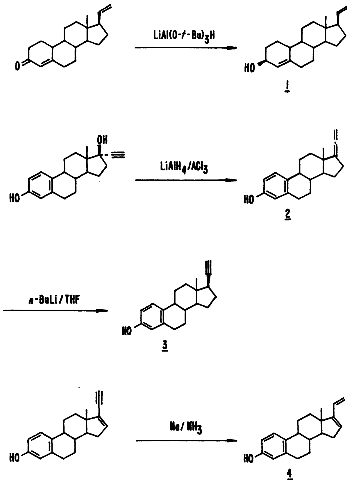
Scheme 1. Syntheses of 19-norpregnanes.
