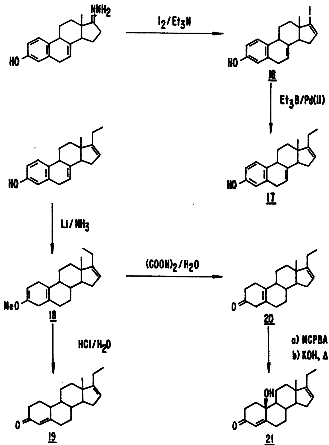
Scheme 5. Pd(II)-catalyzed synthesis of 19-norpregnenes.
