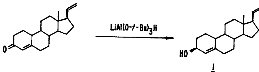
Scheme 1. Syntheses of 19-norpregnanes.
