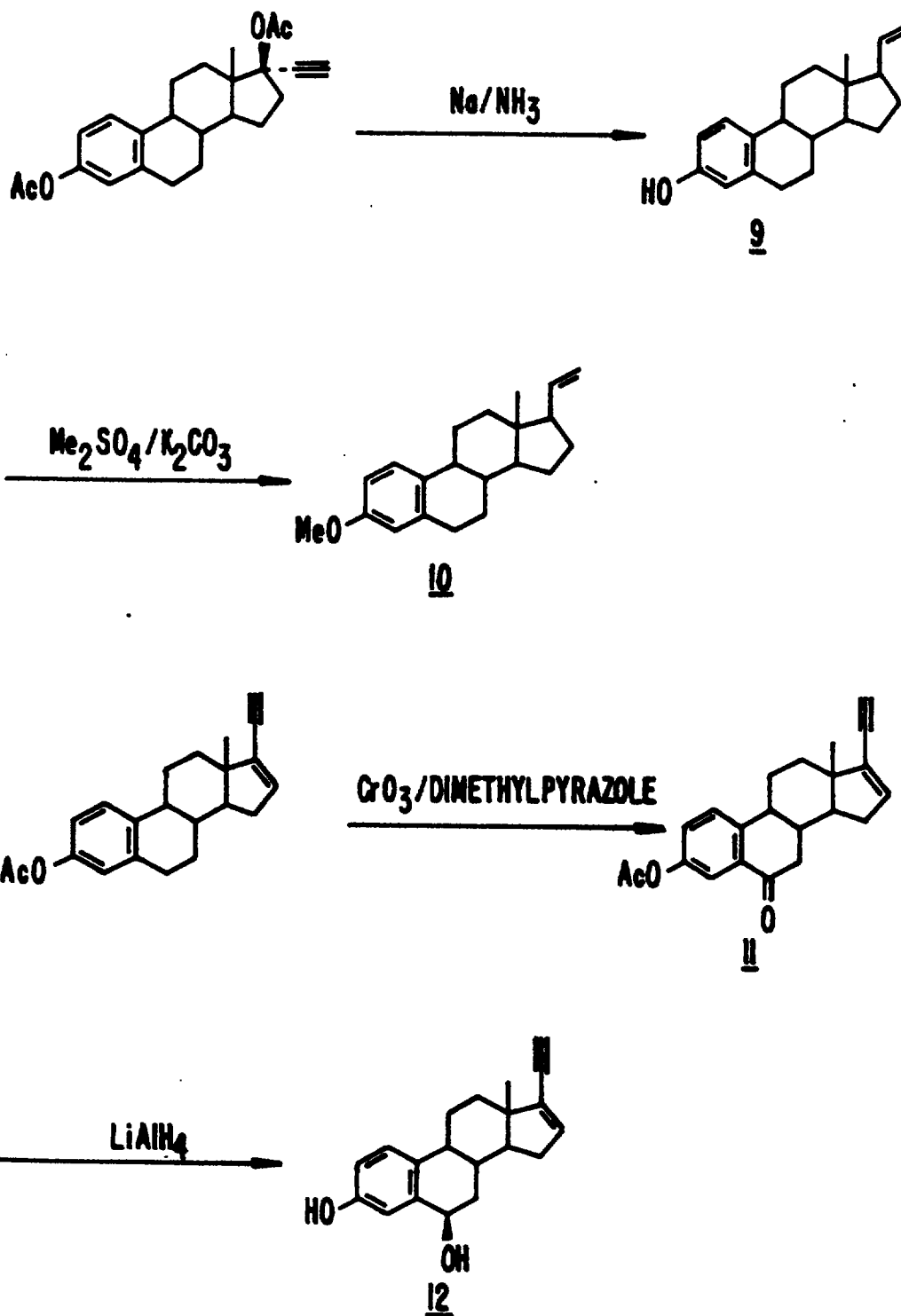
Scheme 3. Further syntheses of norpregnanes.
