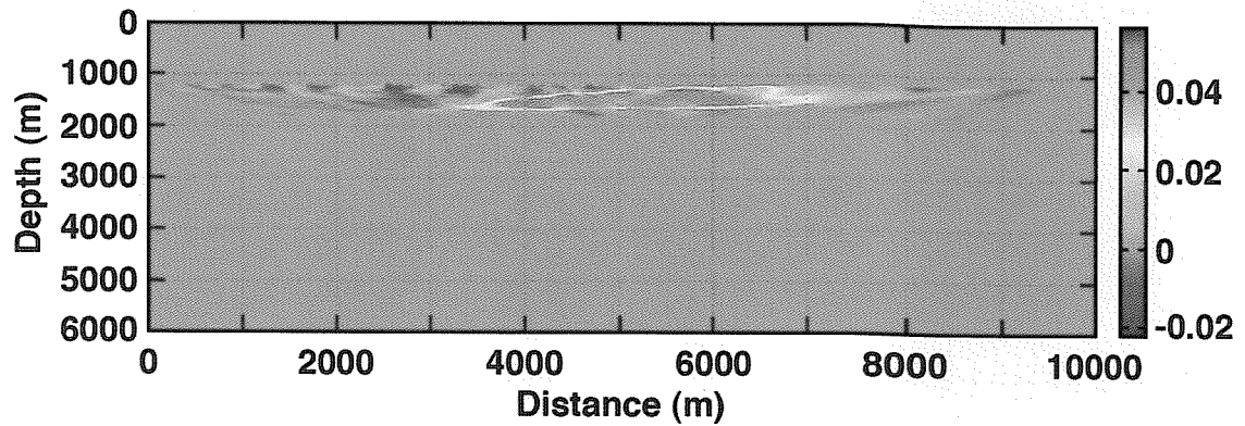
Reconstructed 1/Q Model with f^n \cdot \exp(f/f_0) , Unconstrained Optimization
