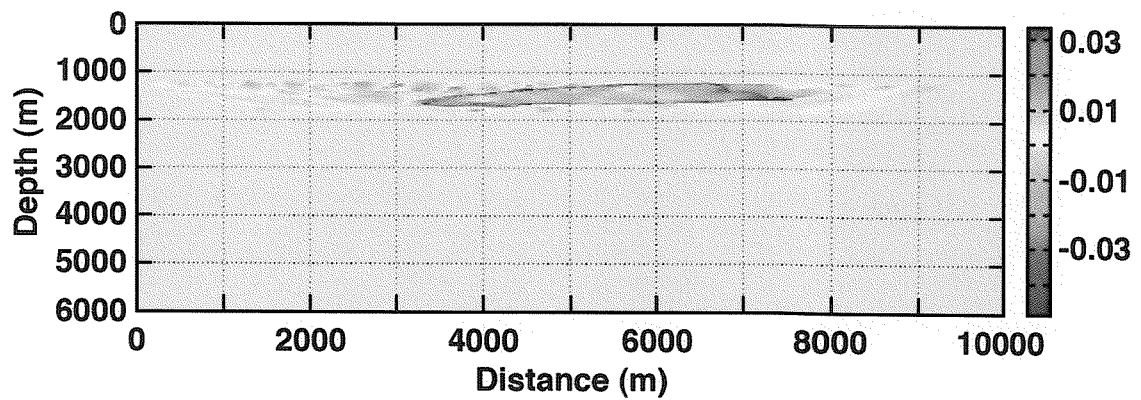
Error of Reconstructed 1/Q Model
