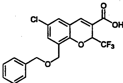
6-Chloro-8-(benzyloxymethyl)-2-(trifluoromethyl)- 2H-1-benzopyran-3-carboxylic acid
