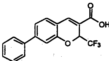
10 7-Phenyl-2-trifluoromethyl-2H-1-benzopyran-3- carboxylic acid
