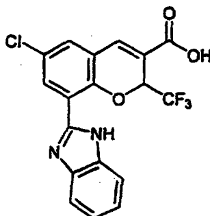
8-(1H-Benzimidazol-2-yl)-6-chloro-2- (trifluoromethyl)-2H-1-benzopyran-3-carboxylic acid
