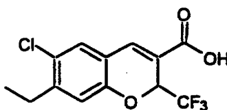
25 6-Chloro-7-ethyl-2-trifluoromethyl-2H-1- benzopyran-3-carboxylic acid
