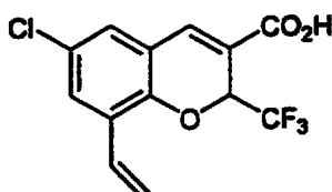
6-Chloro-8-ethenyl-2-(trifluoromethyl)-2H-1- benzopyran-3-carboxylic acid
