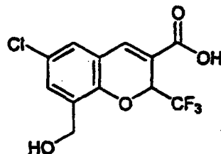
6-Chloro-8-(hydroxymethyl)-2-(trifluoromethyl)- 2H-1-benzopyran-3-carboxylic acid
