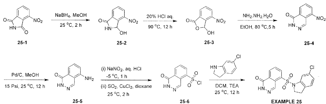
5-((6-Chloroindolin-1-yl)sulfonyl)phthalazin-1(2H)-one
