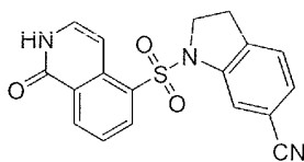
1-((1-Oxo-1,2-dihydroisoquinolin-5-yl)sulfonyl)indoline-6-carbonitrile
