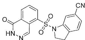
1-((1-Oxo-1,2-dihydrophthalazin-5-yl)sulfonyl)indoline-6-carbonitrile
