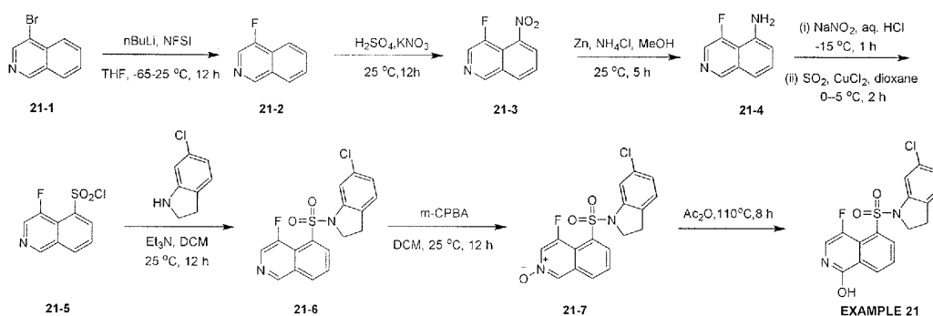
5-((6-Chloroindolin-1-yl)sulfonyl)-4-fluoroisoquinolin-1-ol
