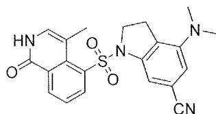
4-(dimethylamino)-1-((4-methyl-1-oxo-1,2-dihydroisoquinolin-5-yl)sulfonyl)indoline-6-carbonitrile
