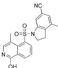
1-((1-Hydroxy-4-methylisoquinolin-5-yl)sulfonyl)-4-methylindoline-6-carbonitrile
