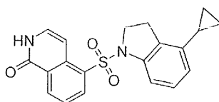
5-((4-Cyclopropylindolin-1-yl)sulfonyl)isoquinolin-1(2H)-one
