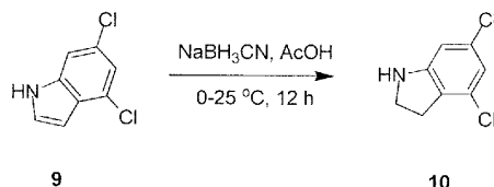
4,6-Dichloroindoline
