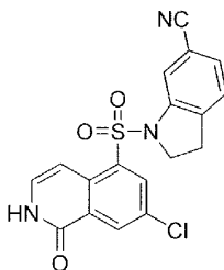
1-((7-Chloro-1-oxo-1,2-dihydroisoquinolin-5-yl)sulfonyl)indoline-6-carbonitrile
