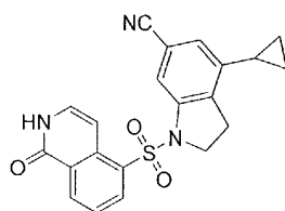
4-Cyclopropyl-1-((1-oxo-1,2-dihydroisoquinolin-5-yl)sulfonyl)indoline-6-carbonitrile
