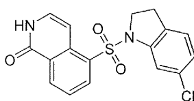
5-((6-Chloroindolin-1-yl)sulfonyl)isoquinolin-1(2H)-one
