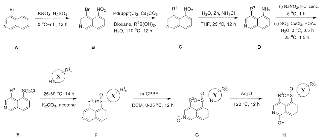
Scheme II
