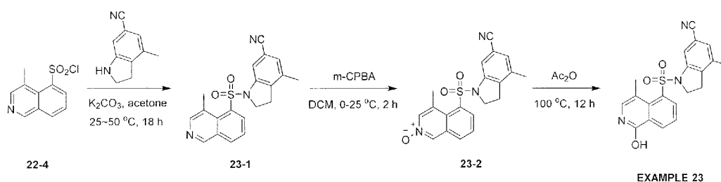
1-((1-Hydroxy-4-methylisoquinolin-5-yl)sulfonyl)-4-methylindoline-6-carbonitrile
