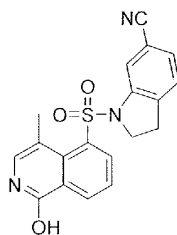
1-((1-Hydroxy-4-methylisoquinolin-5-yl)sulfonyl)indoline-6-carbonitrile
