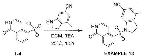
4-Methyl-1-((1-oxo-1,2-dihydroisoquinolin-5-yl)sulfonyl)indoline-6-carbonitrile
