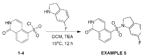
5-((6-Fluoroindolin-1-yl)sulfonyl)isoquinolin-1(2H)-one
