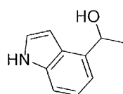
1-(1H-Indol-4-yl)ethan-1-ol
