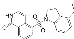
5-((4-ethylindolin-1-yl)sulfonyl)isoquinolin-1(2H)-one
