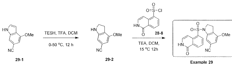
4-methoxy-1-((1-oxo-1,2-dihydroisoquinolin-5-yl)sulfonyl)indoline-6-carbonitrile
