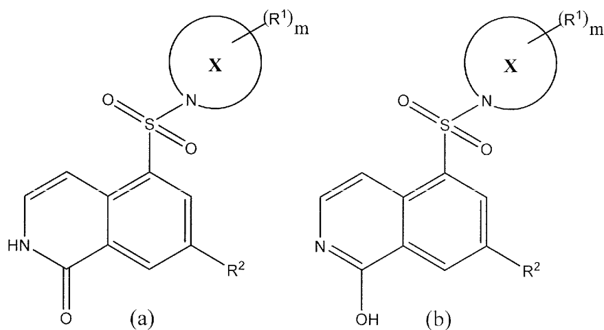
Formula (I)
