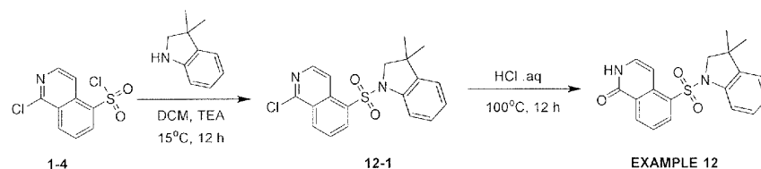
5-((3,3-Dimethylindolin-1-yl)sulfonyl)isoquinolin-1(2H)-one
