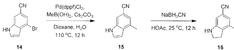
4-Methylindoline-6-carbonitrile
