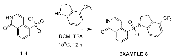
5-((4-(Trifluoromethyl)indolin-1-yl)sulfonyl)isoquinolin-1(2H)-one
