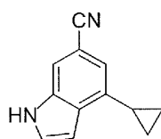
4-Cyclopropyl-1H-indole-6-carbonitrile
