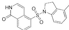
5-((4-Methylindolin-1-yl)sulfonyl)isoquinolin-1(2H)-one
