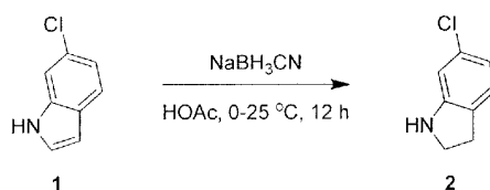
6-Chloroindoline
