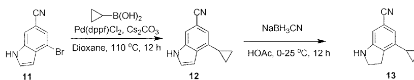
4-Cyclopropylindoline-6-carbonitrile
