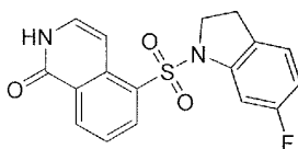
5-((6-Fluoroindolin-1-yl)sulfonyl)isoquinolin-1(2H)-one
