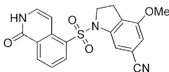
4-methoxy-1-((1-oxo-1,2-dihydroisoquinolin-5-yl)sulfonyl)indoline-6-carbonitrile
