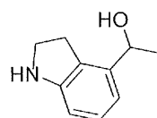
1-(Indolin-4-yl)ethan-1-ol
