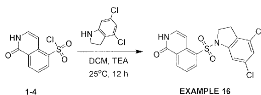
5-((4,6-Dichloroindolin-1-yl)sulfonyl)isoquinolin-1(2H)-one
