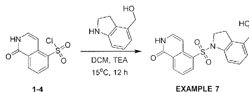
5-((4-(Hydroxymethyl)indolin-1-yl)sulfonyl)isoquinolin-1(2H)-one
