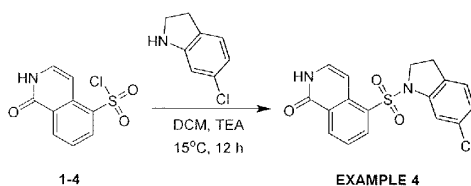
5-((6-Chloroindolin-1-yl)sulfonyl)isoquinolin-1(2H)-one
