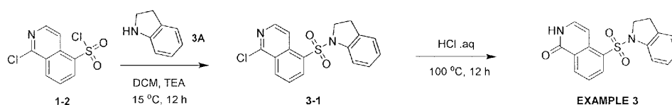
5-(Indolin-1-ylsulfonyl)isoquinolin-1(2H)-one
