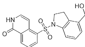
5-((4-(Hydroxymethyl)indolin-1-yl)sulfonyl)isoquinolin-1(2H)-one
