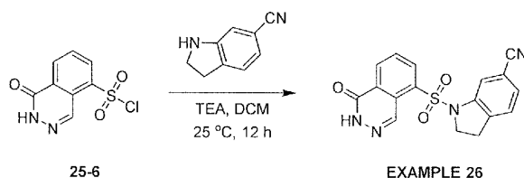
1-((1-Oxo-1,2-dihydrophthalazin-5-yl)sulfonyl)indoline-6-carbonitrile
