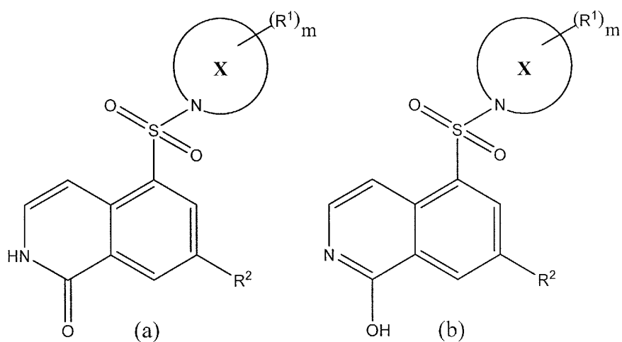
Formula (I)
