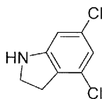
4,6-Dichloroindoline
