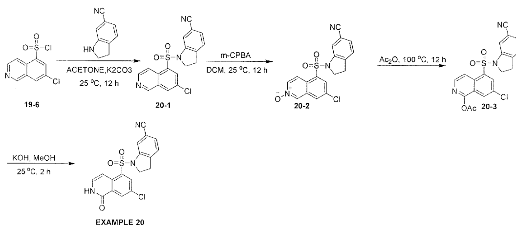
1-((7-Chloro-1-oxo-1,2-dihydroisoquinolin-5-yl)sulfonyl)indoline-6-carbonitrile
