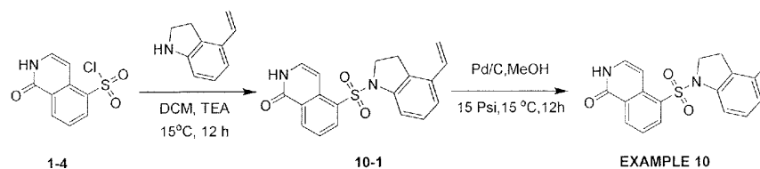
5-((4-ethylindolin-1-yl)sulfonyl)isoquinolin-1(2H)-one
