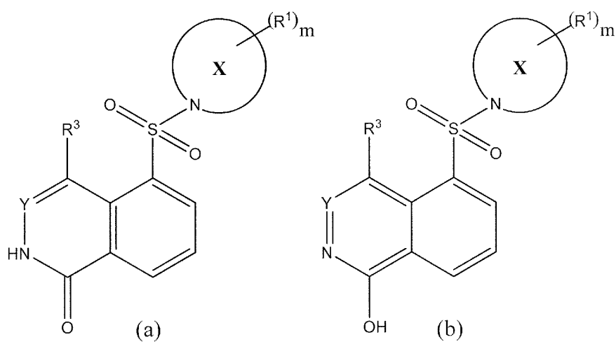
Formula (II)
