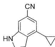
4-Cyclopropylindoline-6-carbonitrile
