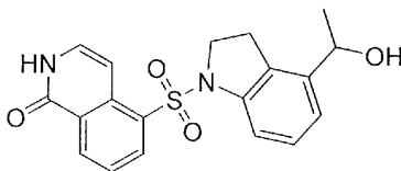
5-((4-(1-Hydroxyethyl)indolin-1-yl)sulfonyl)isoquinolin-1(2H)-one
