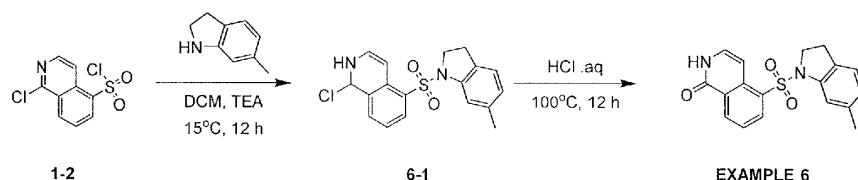
5-((6-Methylindolin-1-yl)sulfonyl)isoquinolin-1(2H)-one
