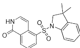
5-((3,3-Dimethylindolin-1-yl)sulfonyl)isoquinolin-1(2H)-one
