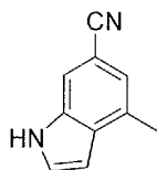
4-Methyl-1H-indole-6-carbonitrile
