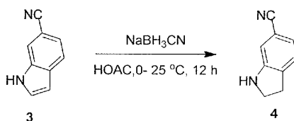
Indoline-6-carbonitrile
