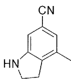
4-Methylindoline-6-carbonitrile
