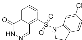
5-((6-Chloroindolin-1-yl)sulfonyl)phthalazin-1(2H)-one
