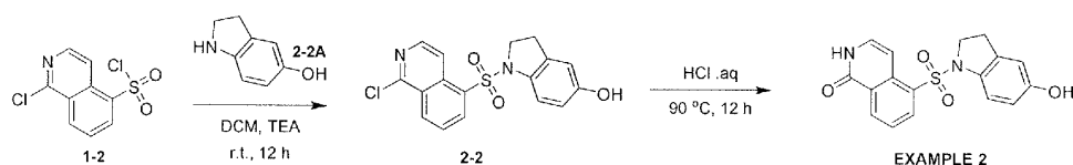
5-((5-Hydroxyindolin-1-yl)sulfonyl)isoquinolin-1(2H)-one
