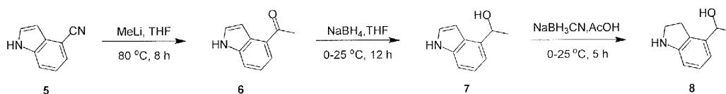
1-(Indolin-4-yl)ethan-1-ol
