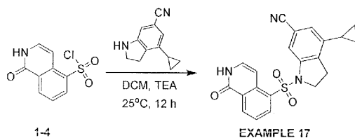
4-Cyclopropyl-1-((1-oxo-1,2-dihydroisoquinolin-5-yl)sulfonyl)indoline-6-carbonitrile
