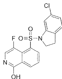
5-((6-Chloroindolin-1-yl)sulfonyl)-4-fluoroisoquinolin-1-ol
