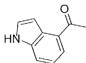
1-(1H-Indol-4-yl)ethan-1-one
