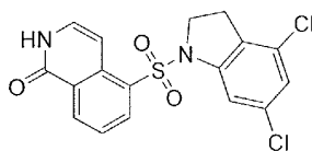
5-((4,6-Dichloroindolin-1-yl)sulfonyl)isoquinolin-1(2H)-one
