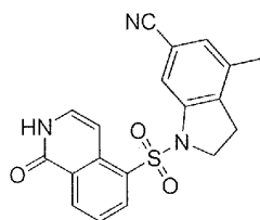
4-Methyl-1-((1-oxo-1,2-dihydroisoquinolin-5-yl)sulfonyl)indoline-6-carbonitrile
