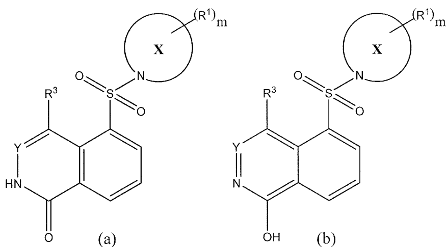
Formula (II)
