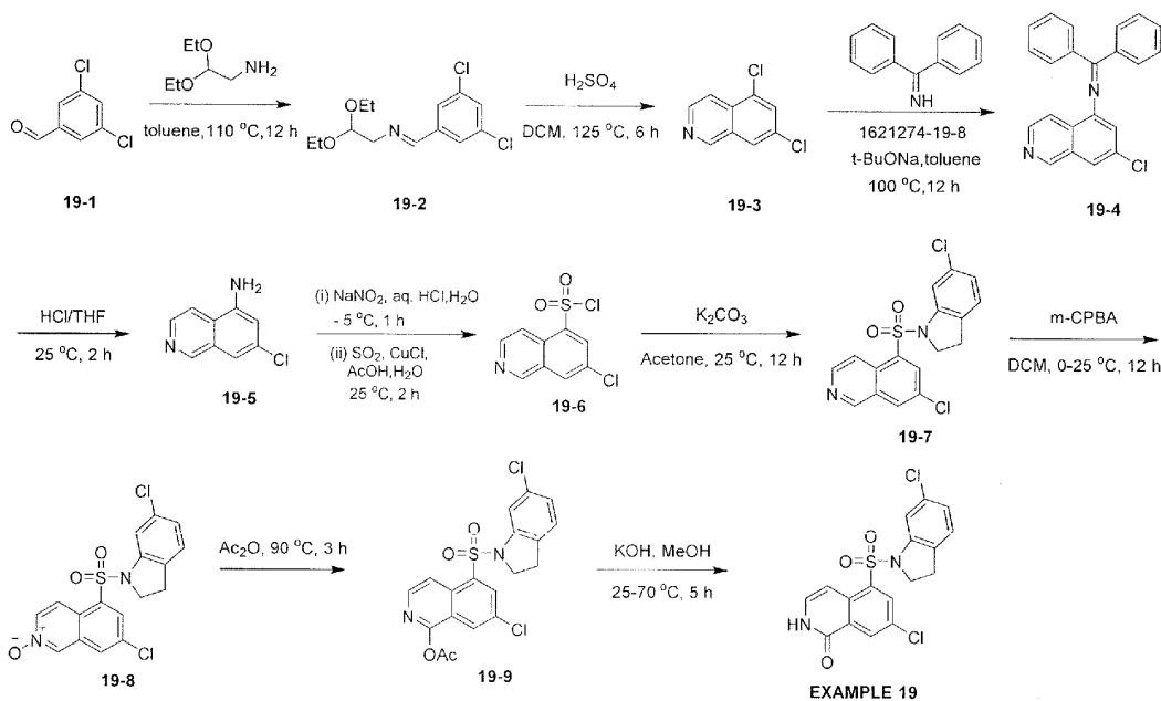
7-Chloro-5-((6-chloroindolin-1-yl)sulfonyl)isoquinolin-1(2H)-one
