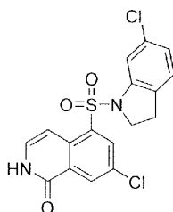
7-Chloro-5-((6-chloroindolin-1-yl)sulfonyl)isoquinolin-1(2H)-one
