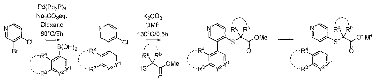
Scheme I-B-b:
