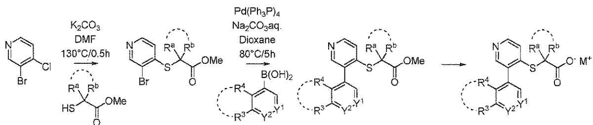
10 Scheme I-B-c:
