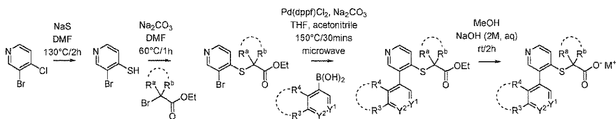
Scheme I-B-a:
