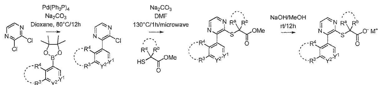
Scheme I-E-a:
