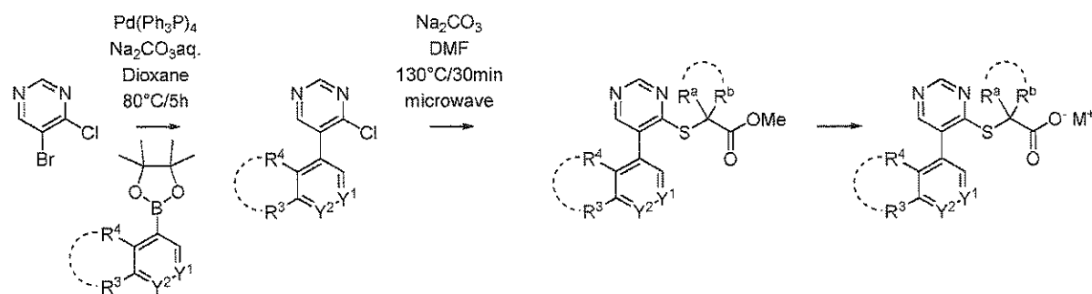
Scheme I-F-b:
