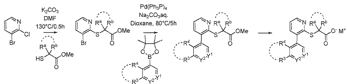
Scheme I-E-a:
