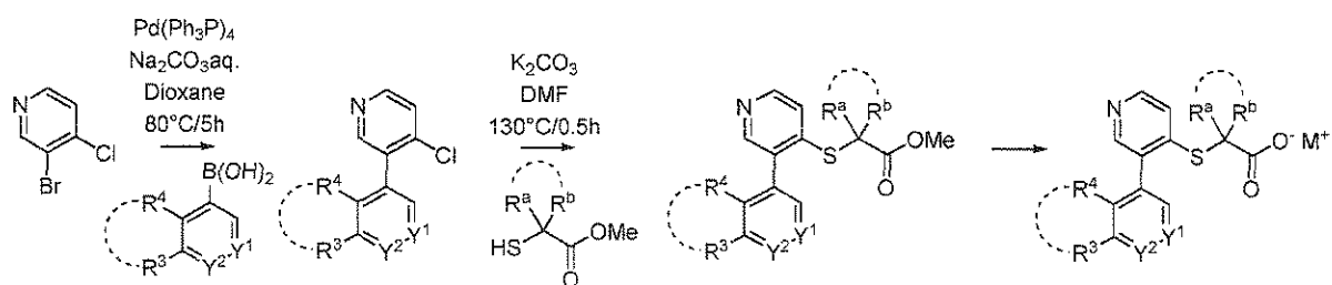
Scheme I-B-b:
