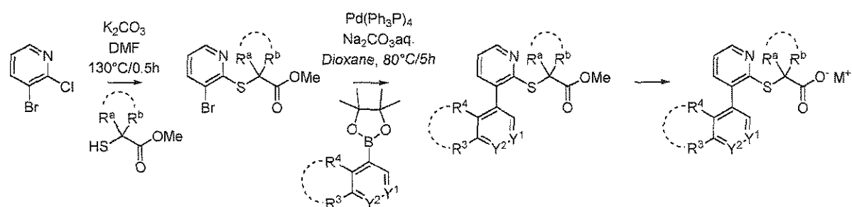
Scheme I-D-c:
