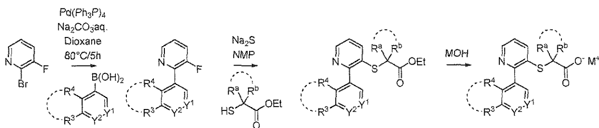
Scheme I-A-b:
