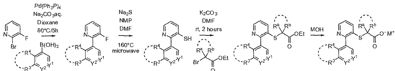
Scheme I-A-b:
