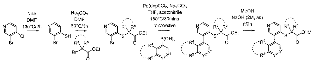
Scheme I-B-b:
