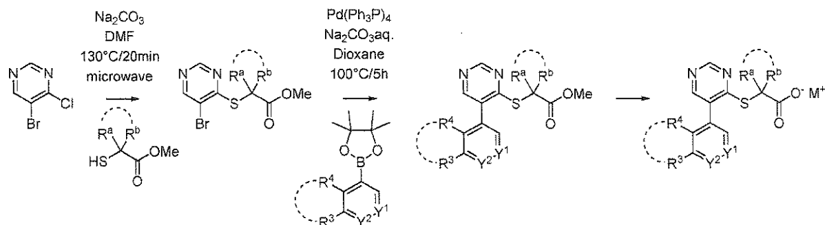
Scheme I-F-a:
