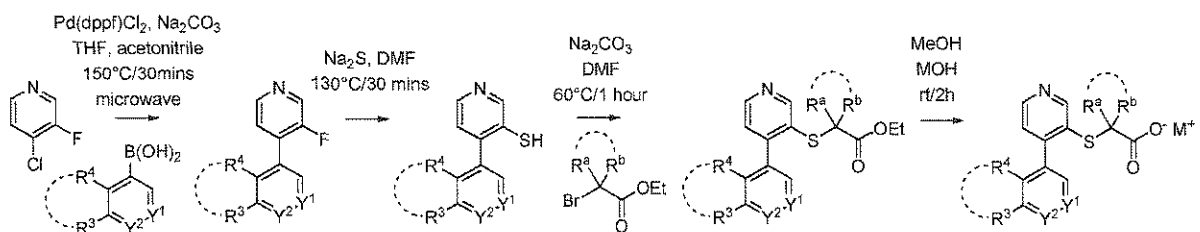
Scheme I-C:
