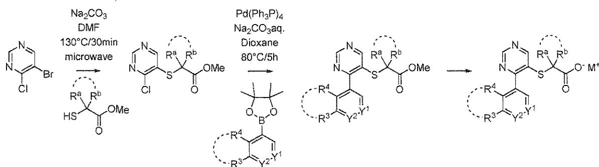
Scheme I-H-a:
