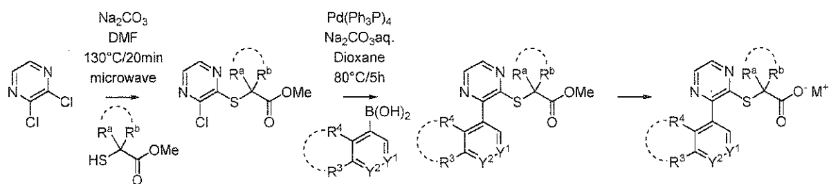
Scheme I-F-a:
