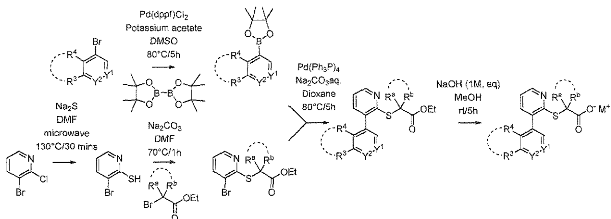
Scheme I-D-a:
