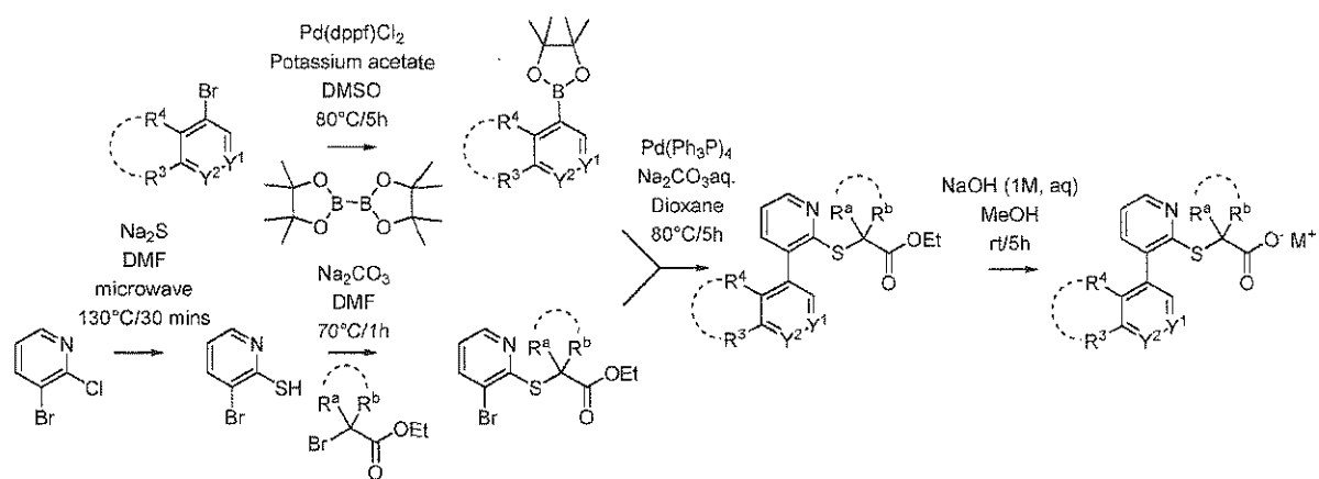
Scheme I-D-b:
