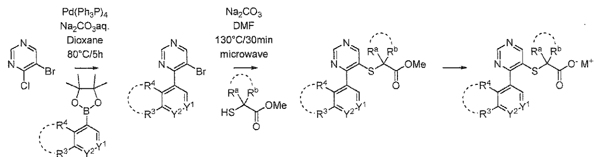
Scheme I-G-a:
