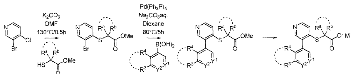
Scheme I-B-c:
