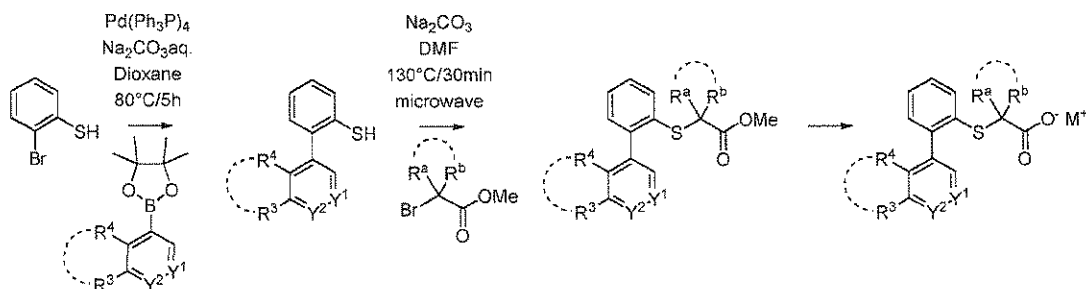
Scheme I-H-a:
