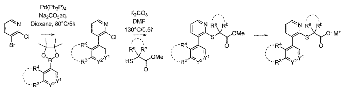
Scheme I-D-b:
