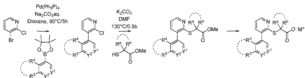
Scheme I-D-c:
