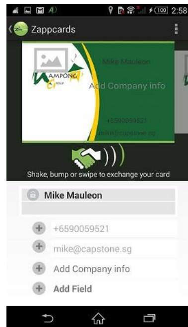
Figure 6 - Sending Screen
