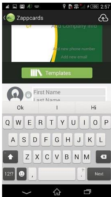
Figure 5 - Template Screen
