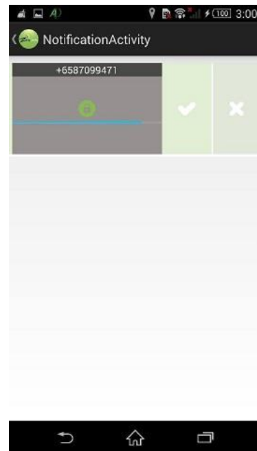
Figure 8 - Notification Screen
