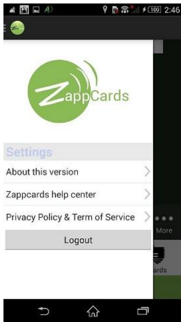
Figure 11 - Settings Screen
