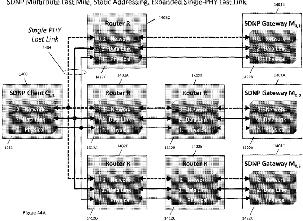
SDNP Multiroute Last Mile, Static Addressing, Expanded Single-PHY Last Link
