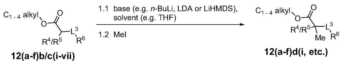
Scheme 7d
