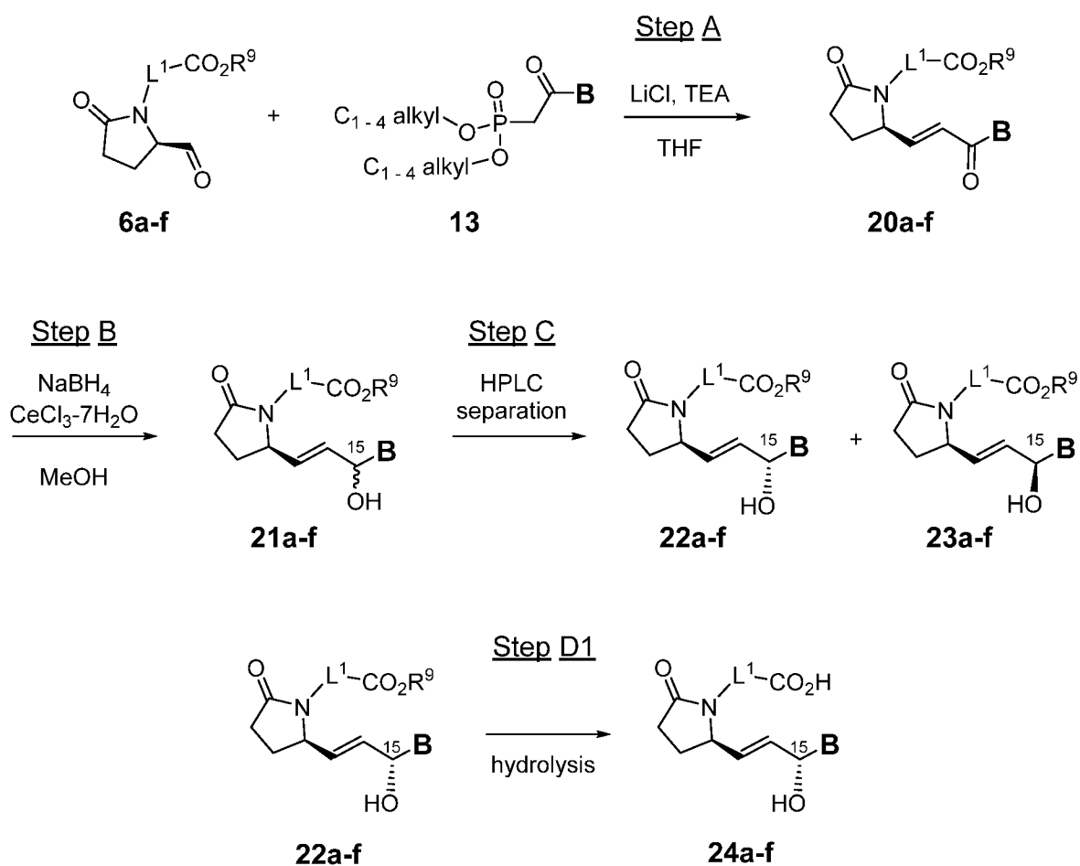
Scheme 9
