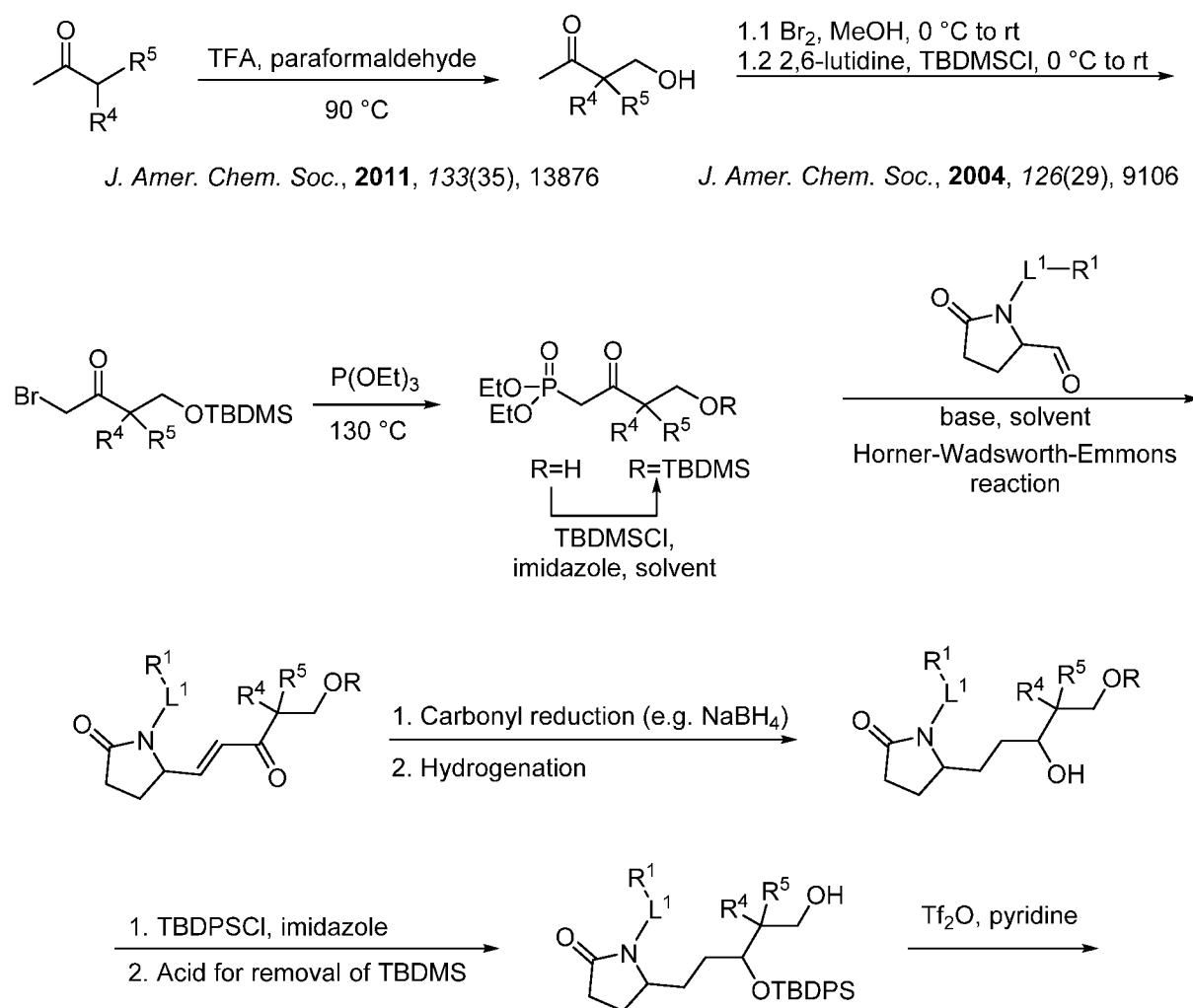
Scheme 1C
