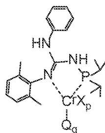
Structure CrGu II
