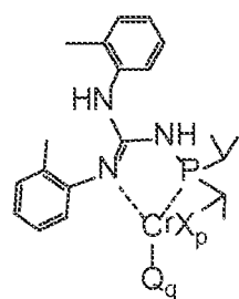
Structure CrGu I
