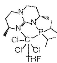
Structure \text{CrCl}_3 \cdot \text{THF} Gu XIII
