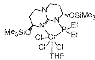
Structure \text{CrCl}_3 \cdot \text{THF} Gu XVI
