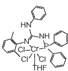
Structure CrCl 3 • THF Gu III
