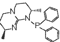
Structure Gu XIV
