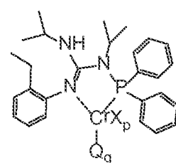
Structure CrGu XX
