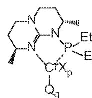
Structure CrGu XII
