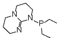
Structure Gu XXIII
