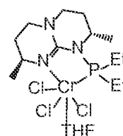
Structure \text{CrCl}_3 \cdot \text{THF} Gu XII
