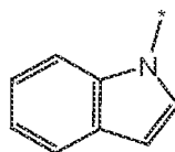
indol-1-yl “arylheteryl group”
