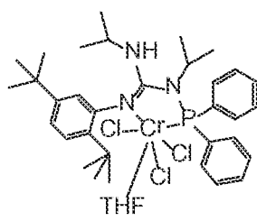
Structure \text{CrCl}_3 \cdot \text{THF} Gu XXII
