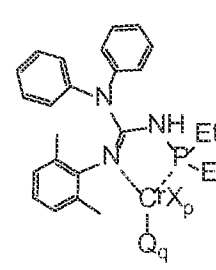
Structure CrGu IV
