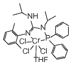
Structure \text{CrCl}_3 \cdot \text{THF} Gu XIX
