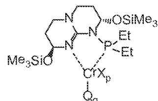
Structure CrGu XVI
