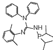
Structure Gu V
