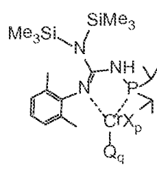
Structure CrGu VI
