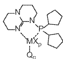
Structure MGu IX
