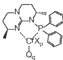
Structure CrGu XIV
