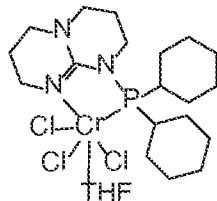
Structure \text{CrCl}_3 \cdot \text{THF} Gu X
