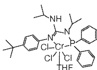
Structure \text{CrCl}_3 \cdot \text{THF} Gu XXI
