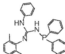
Structure Gu III
