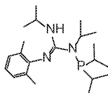
Structure Gu XVIII
