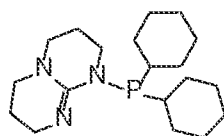
Structure Gu X
