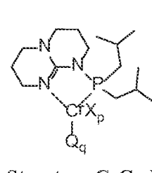
Structure CrGu VIII
