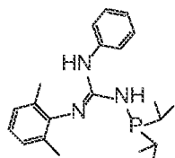
Structure Gu II
