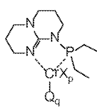
Structure CrGu XXIII
