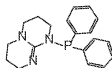
Structure Gu XI
