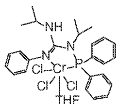
Structure \text{CrCl}_3 \cdot \text{THF} Gu XVII
