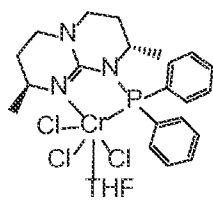
Structure \text{CrCl}_3 \cdot \text{THF} Gu XIV
