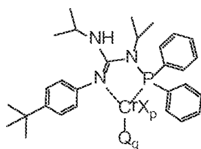
Structure CrGu XXI
