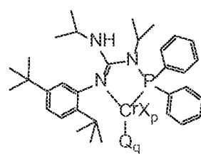
Structure CrGu XXII
