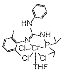
Structure CrCl 3 • THF Gu II
