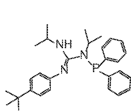
Structure Gu XXI
