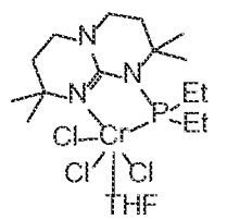
Structure \text{CrCl}_3 \cdot \text{THF} Gu XV
