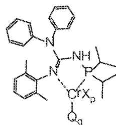
Structure CrGu V
