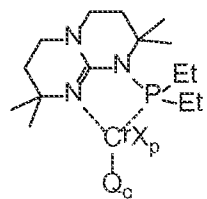
Structure CrGu XV
