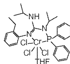
Structure \text{CrCl}_3 \cdot \text{THF} Gu XX
