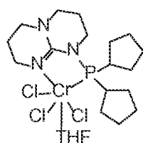
Structure \text{CrCl}_3 \cdot \text{THF} Gu IX
