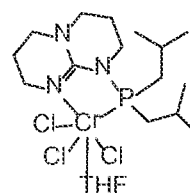
Structure \text{CrCl}_3 \cdot \text{THF} Gu VIII
