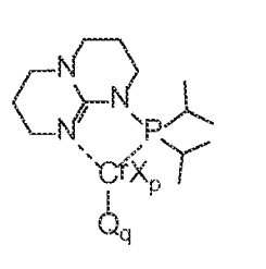
Structure CrGu VII
