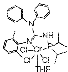
Structure \text{CrCl}_3 \cdot \text{THF} Gu V
