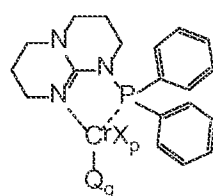
Structure CrGu XI
