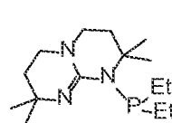
Structure Gu XV
