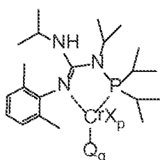
Structure CrGu XVIII
