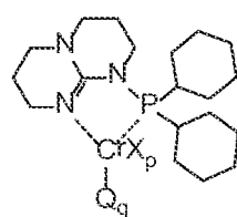
Structure CrGu X
