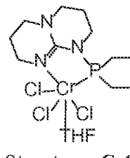
Structure \text{CrCl}_3 \cdot \text{THF} Gu XXIII
