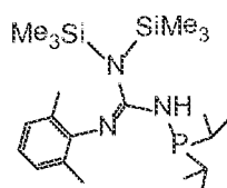
Structure Gu VI
