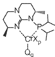
Structure CrGu XIII
