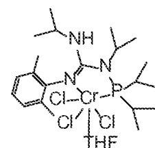
Structure \text{CrCl}_3 \cdot \text{THF} Gu XVIII
