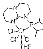
Structure \text{CrCl}_3 \cdot \text{THF} Gu VII
