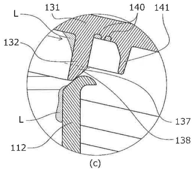
ENLARGED VIEW OF PART K
