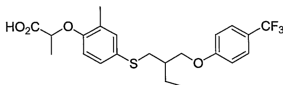
Compound 1
