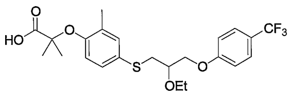
2-{4-[2-Ethoxy-3-(4-trifluoromethyl-phenoxy)-propylsulfanyl]-2-methyl-phenoxy}-2-methyl-propionic acid
