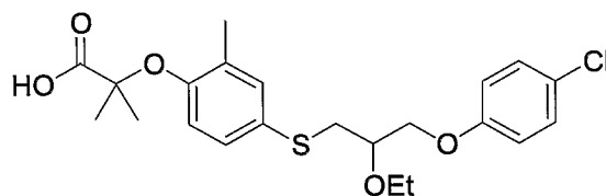
Compound 10
