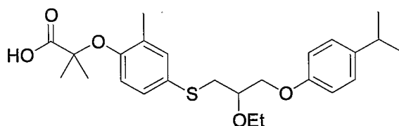
Compound 8
