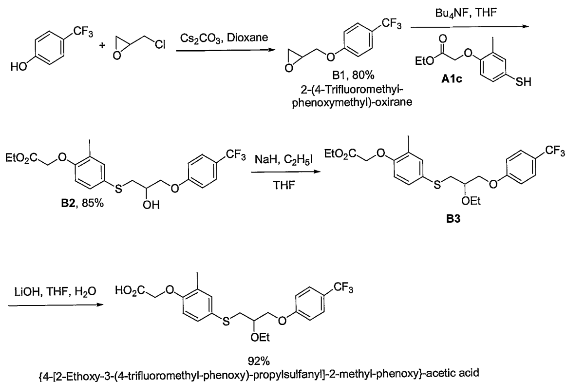
Scheme B
