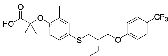
compound 4 #26171158#
