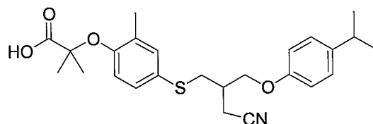
Compound 13
