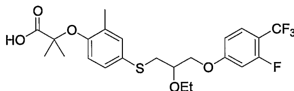
Compound 12
