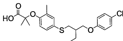
Compound 5
