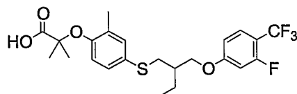
Compound 7
