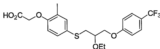
{4-[2-Ethoxy-3-(4-trifluoromethyl-phenoxy)-propylsulfanyl]-2-methyl-phenoxy}-acetic acid
