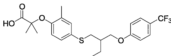
Compound 2
