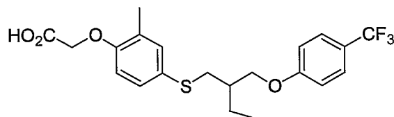
{2-Methyl-4-[2-(4-trifluoromethyl-phenoxy)methyl]-butylsulfanyl}-phenoxy}-acetic acid
