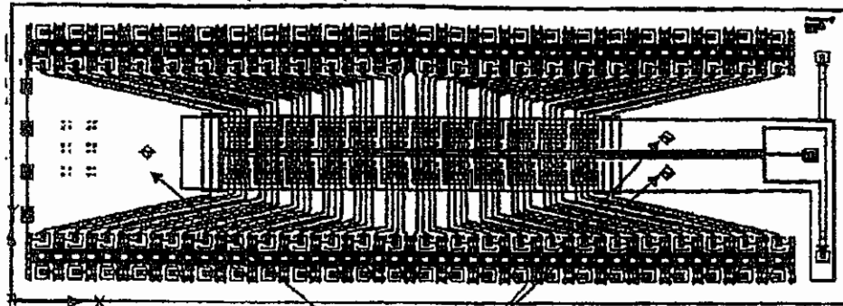
Fiducial Locations on Topaz Microprocessors
