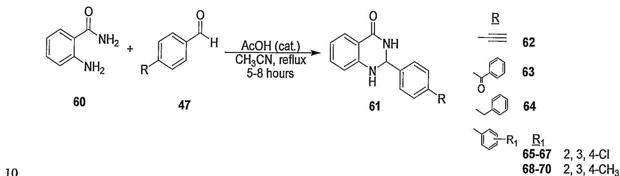
Scheme 6. Synthesis of second generation analogues 62-70.
