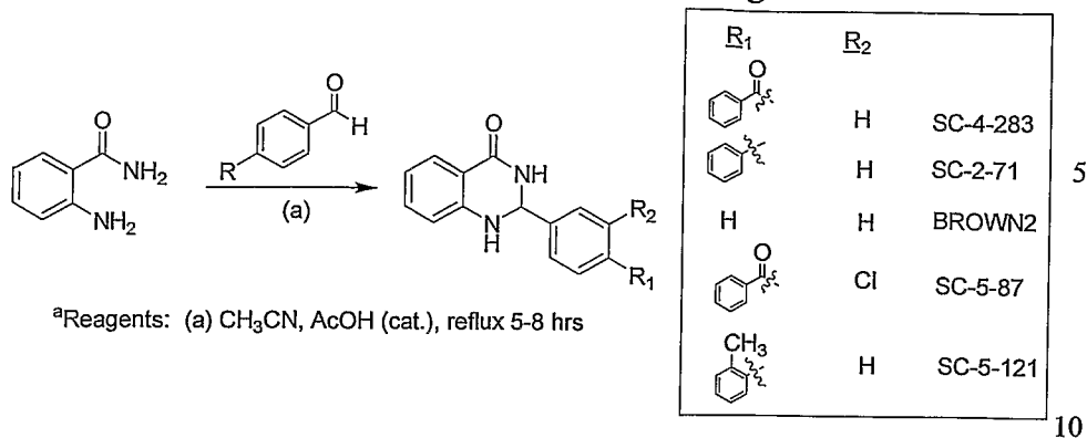
Scheme 1. Synthetic route for SC-2-71 and analogues.
