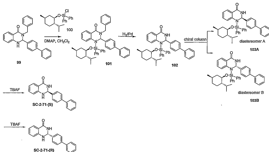
Scheme 12. Chiral resolution of SC-2-71.
