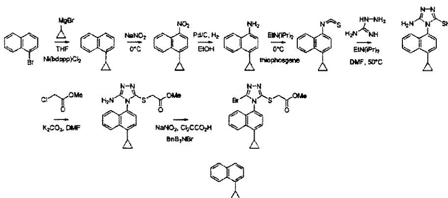
1-Cyclopropylnaphthalene
