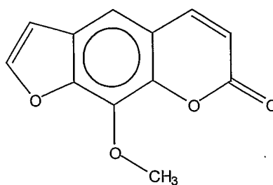
8-Methoxypsoralen
