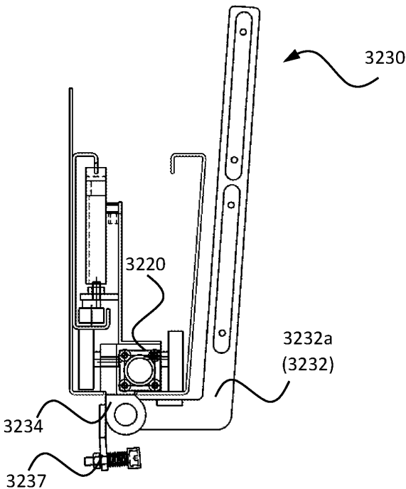
Fig. 12C (VIEW B-B)
