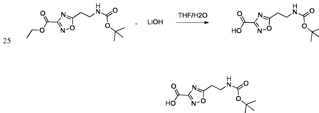
5-(2-((tert-butoxycarbonyl)amino)ethyl)-1,2,4-oxadiazole-3-carboxylic acid
