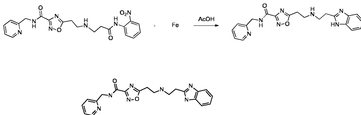
5-(2-((2-(1 H-benzo[ d]imidazol-2-yl)ethyl)amino)ethyl)- N-(pyridin-2-ylmethyl)-1,2,4-oxadiazole-3-carboxamide
