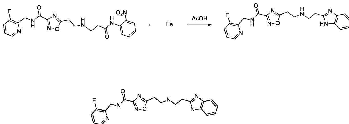
5-(2-((2-(1 H -benzo[ d ]imidazol-2-yl)ethyl)amino)ethyl)- N -((3-fluoropyridin-2-yl)methyl)-1,2,4-oxadiazole-3-carboxamide
