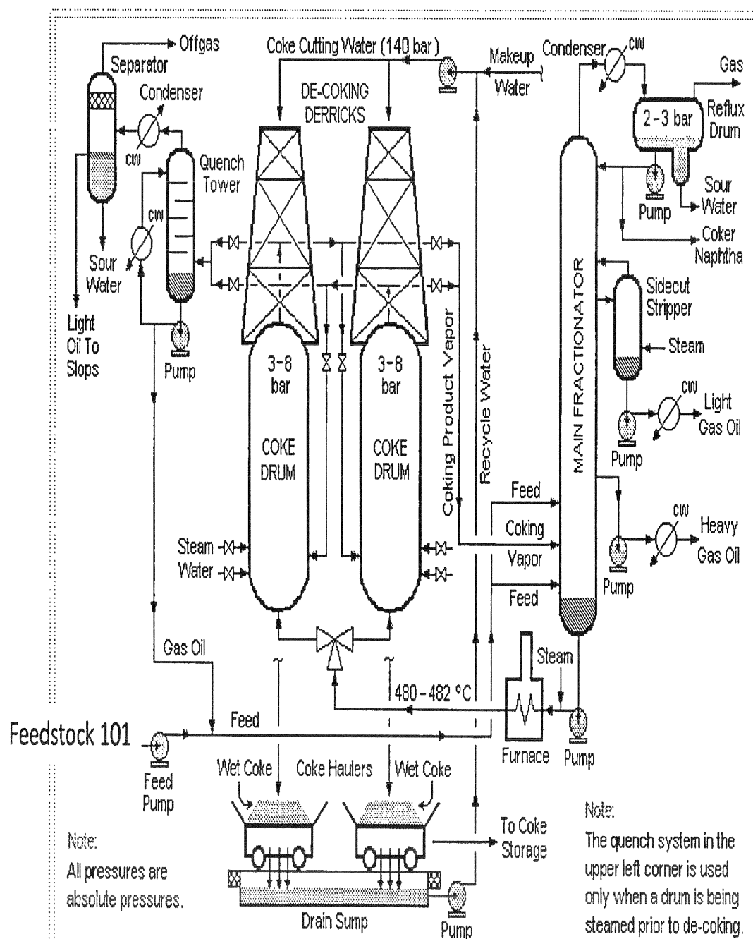
Figure 4 schematic flow diagram of a delayed coking unit
