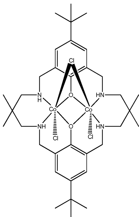
[L^1Co_2Cl_3]^- [B-H]^+
