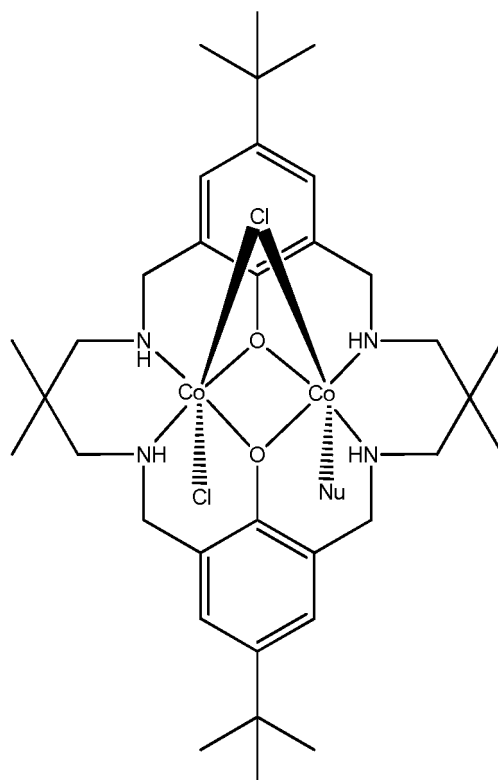
[L^1Co_2Cl_2Nu]
