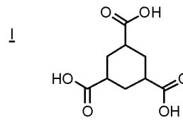
1,3,5-cyclohexanetricarboxylic acid Chemical Formula: C_9H_{12}O_6 Molecular Weight: 216.19
