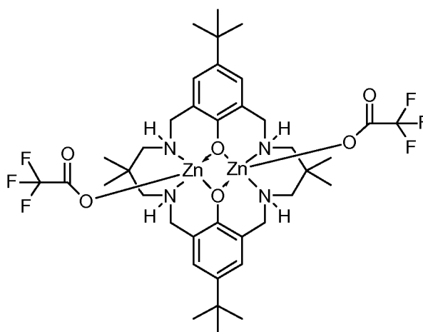
2: [L^1Zn_2(CF_3COO)_2]
