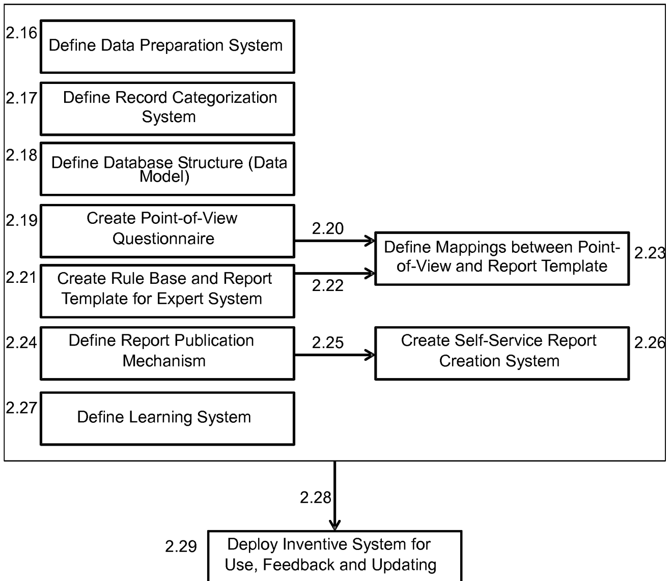
Figure 6: Provisioning Methodology
