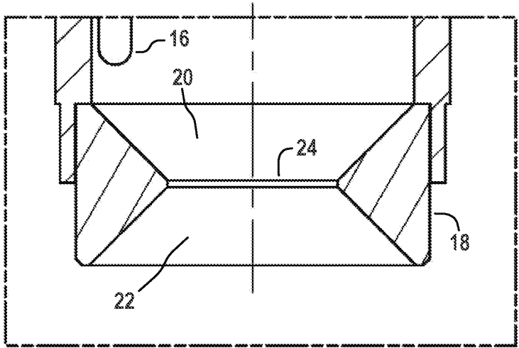
view 2B (detail B)
