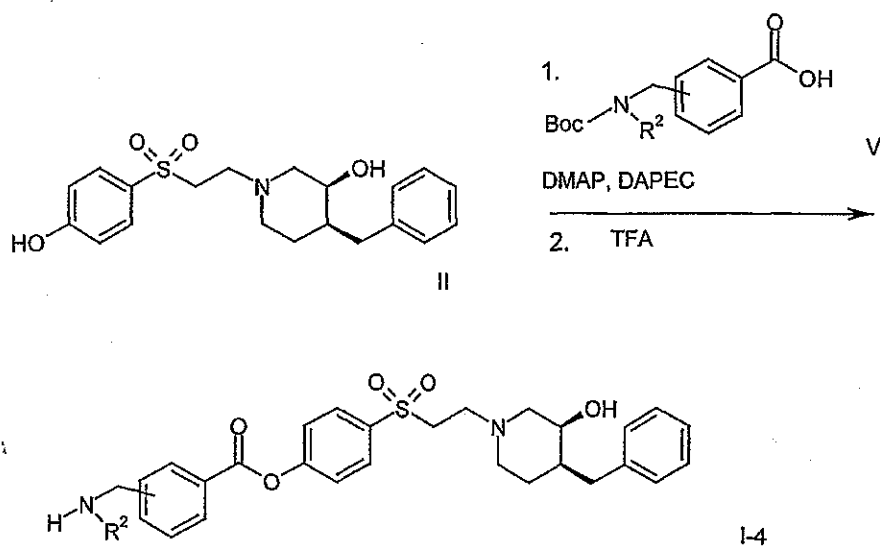
Scheme 3
