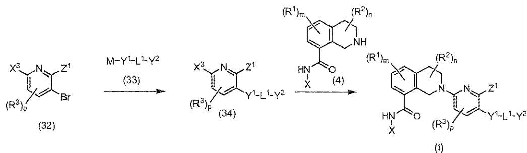
Scheme 7
