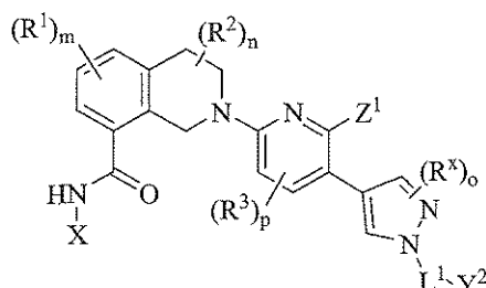
Formula (III),
