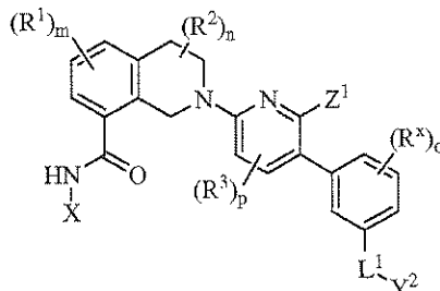
Formula (V),
