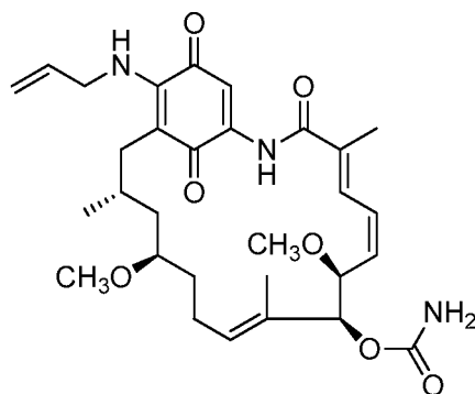
17-(Allylamino)-17-demethoxygeldanamycin
