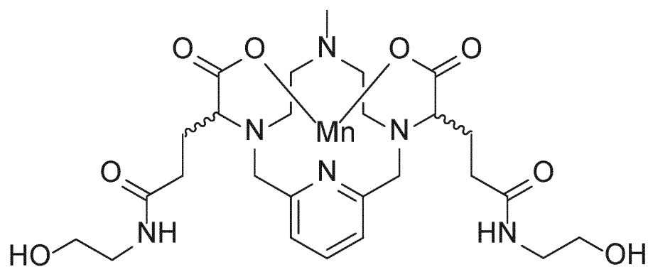
Mn Chelate-15
