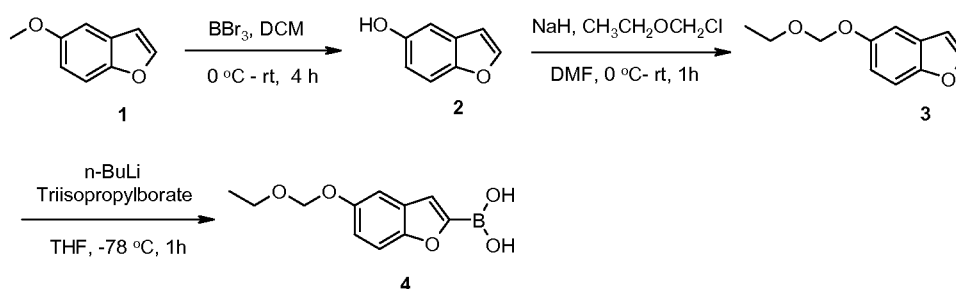
Scheme 1. Synthesis of 5-ethoxymethoxy-benzofuran-2-boronic acid (4)
