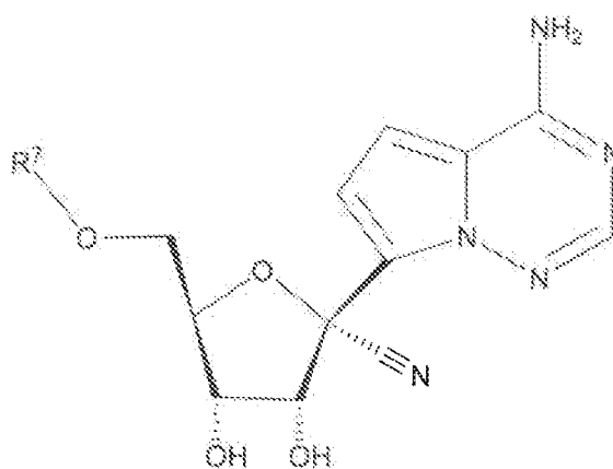
Formula IV
