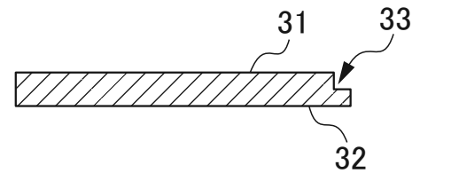
A-A CROSS-SECTIONAL VIEW FIG. 6C
