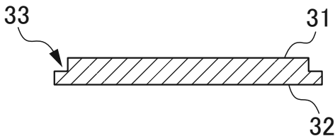
A-A CROSS-SECTIONAL VIEW FIG. 5C
