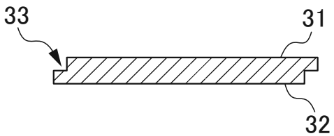
B-B CROSS-SECTIONAL VIEW FIG. 8D
