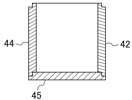
FIG. 11H C-C CROSS-SECTIONAL VIEW
