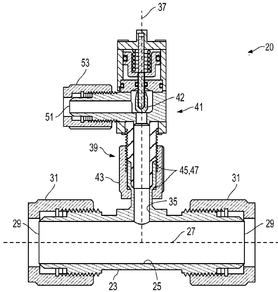
SECTION 9-9
