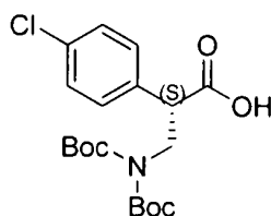
( S )-3-(( bis-tert -butoxycarbonyl)amino)-2-(4-chlorophenyl)propanoic acid
